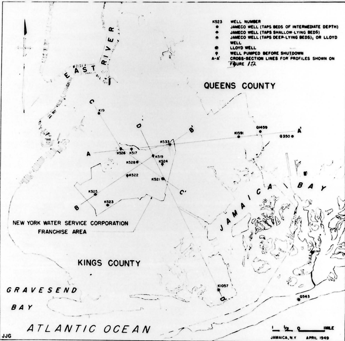
FIGURE 9.—INDEX MAP SHOWING ARTESIAN WELLS AND CROSS-SECTION LINES IN KINGS AND QUEENS COUNTIES, N.Y.
