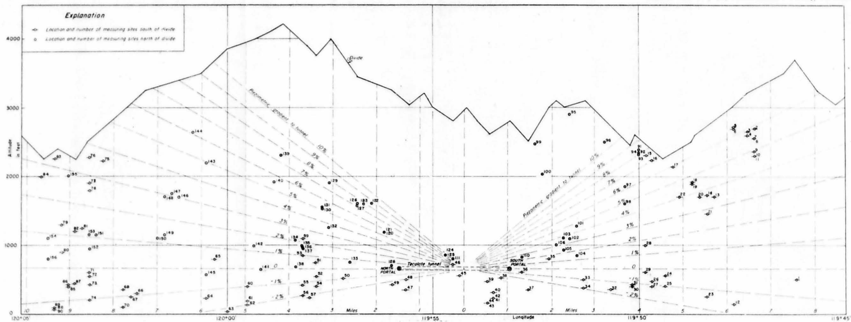
Fig. 2 Altitude and distribution of measuring sites in Tecolote tunnel area, Santa Barbara County, California
