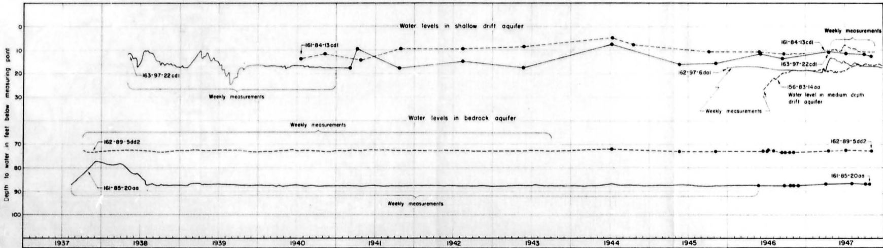
Water-level fluctuation in six wells in the Crosby-Mohall area, North Dakota, 1937 - 1947.
