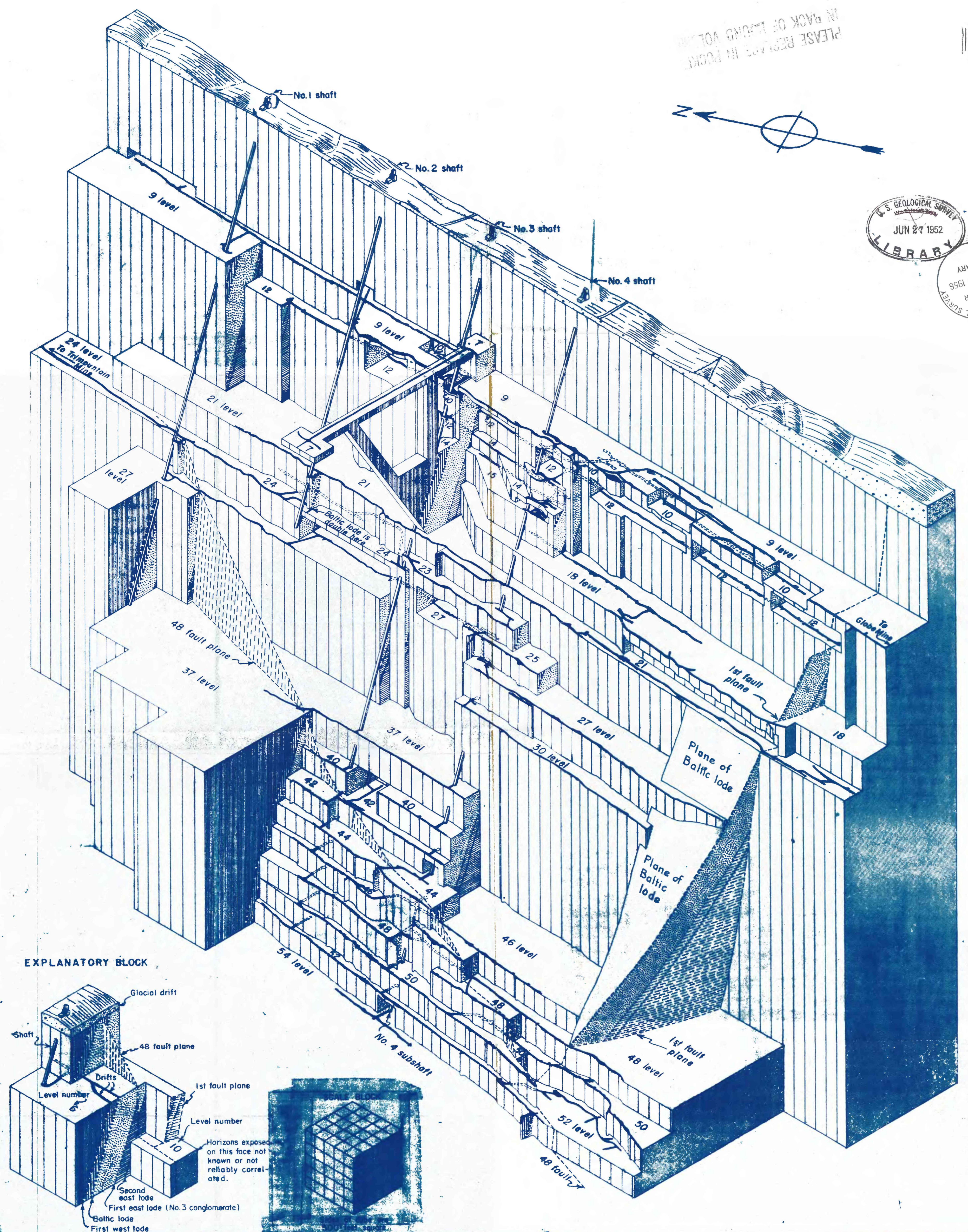
BLOCK DIAGRAM OF ACCESSIBLE WORKINGS, CHAMPION MINE, HOUGHTON COUNTY, MICHIGAN
