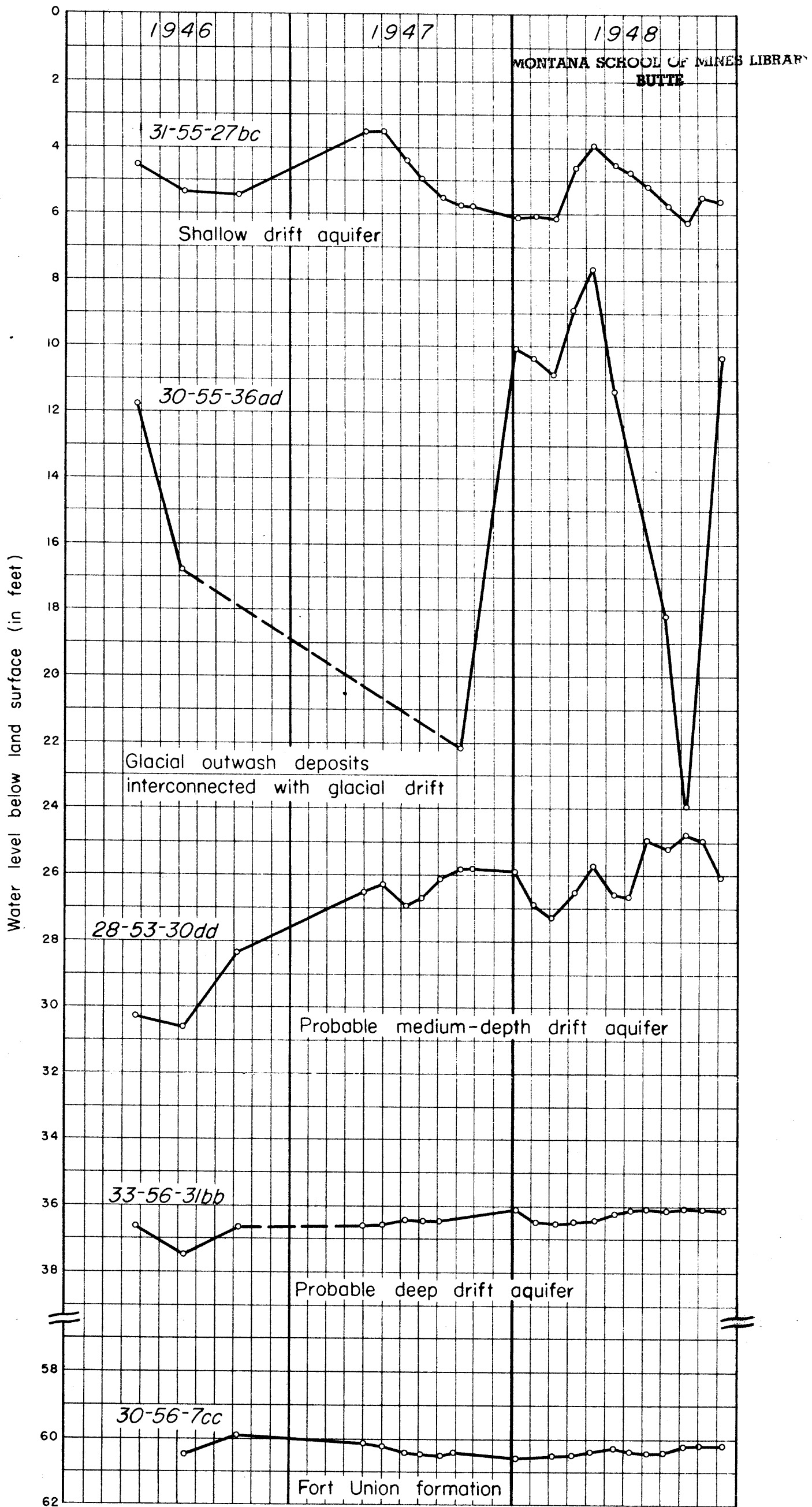
Hydrographs of selected observation wells, Medicine Lake area, Montana
