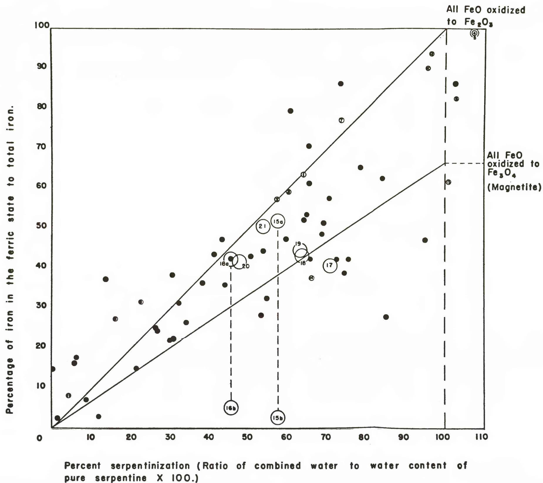
Figure 14, Relationship of state of oxidization of iron to extent of serpentinization in peridotite.
