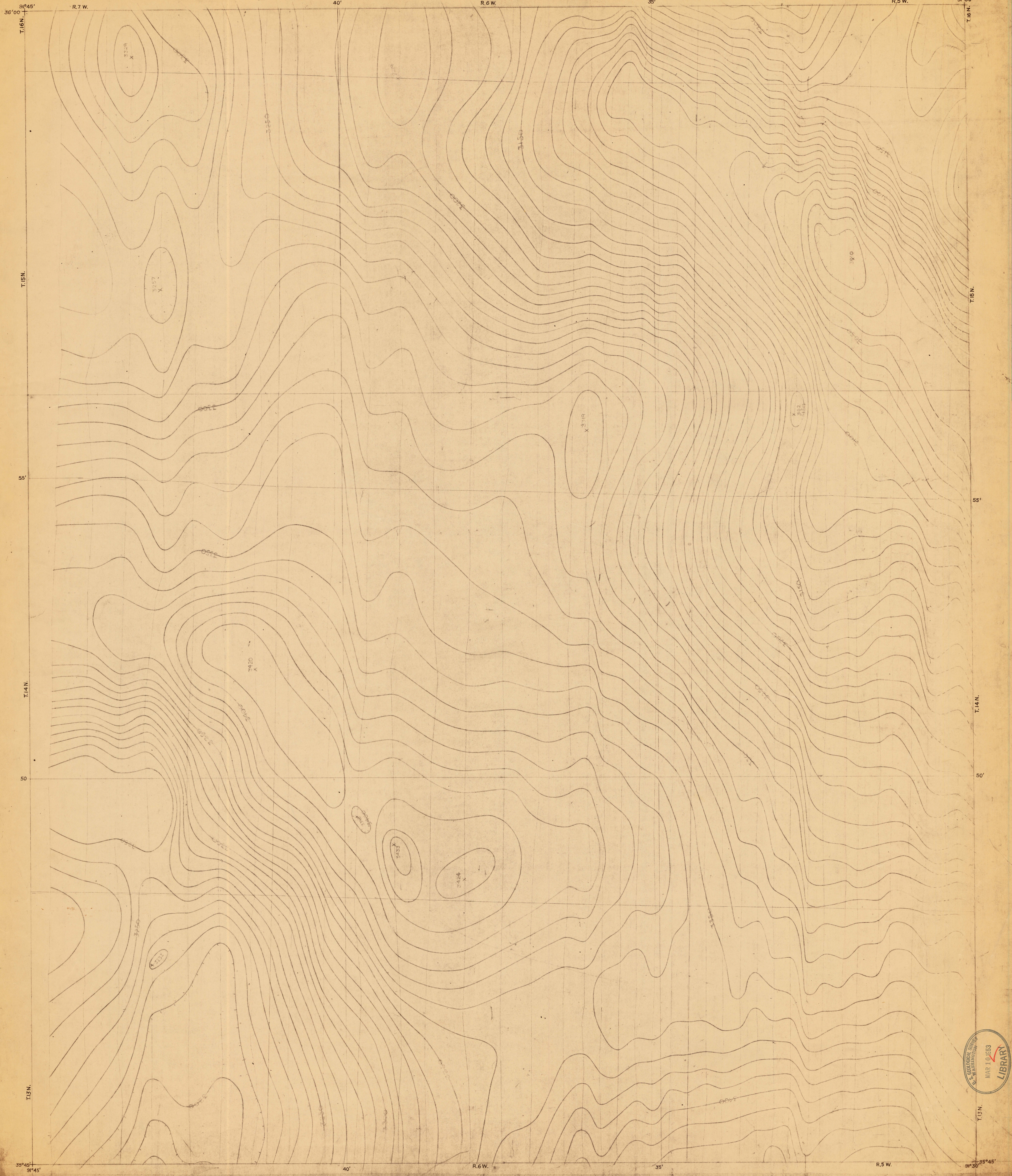
PRELIMINARY TOTAL INTENSITY AEROMAGNETIC MAP OF CAVE CITY QUADRANGLE, ARKANSAS
