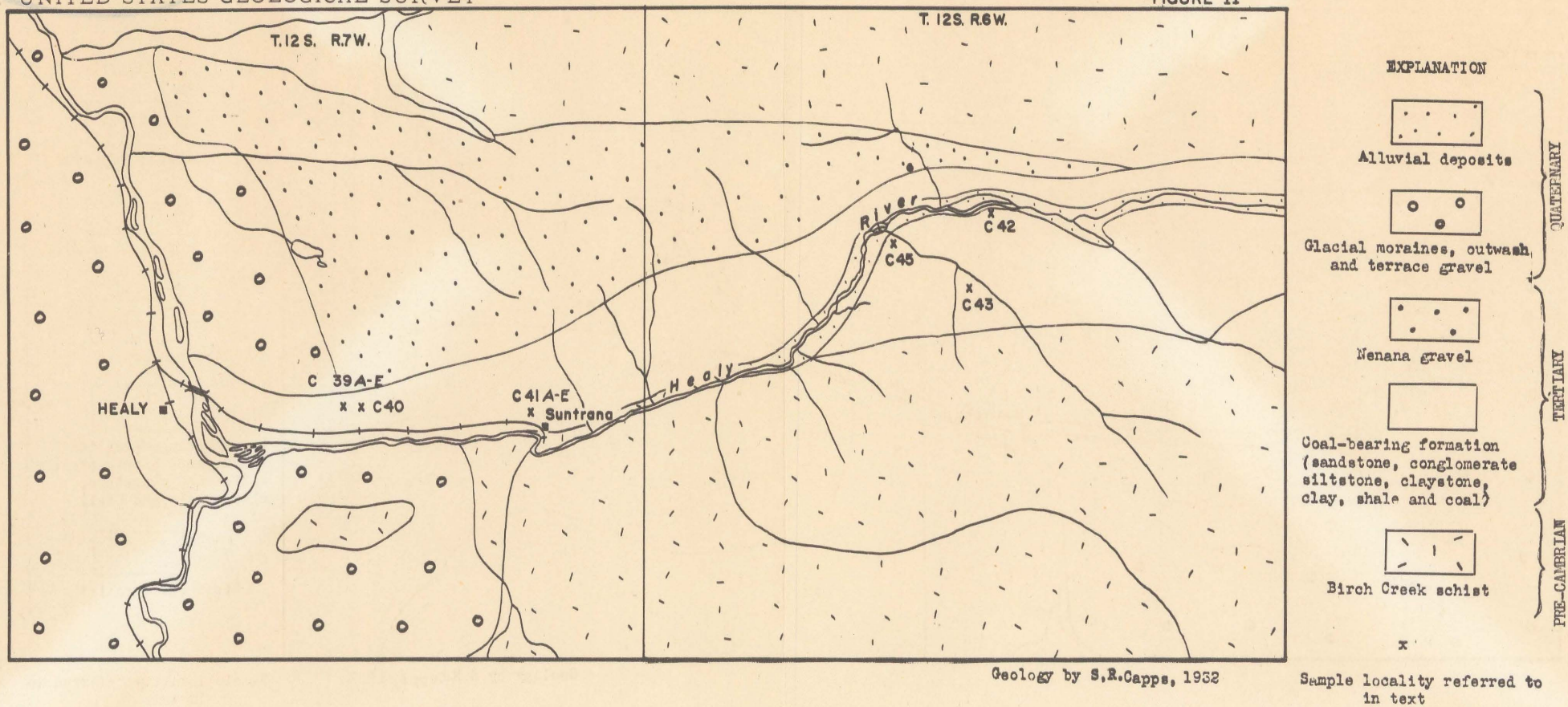
GEOLOGIC MAP OF THE HEALY RIVER AREA
