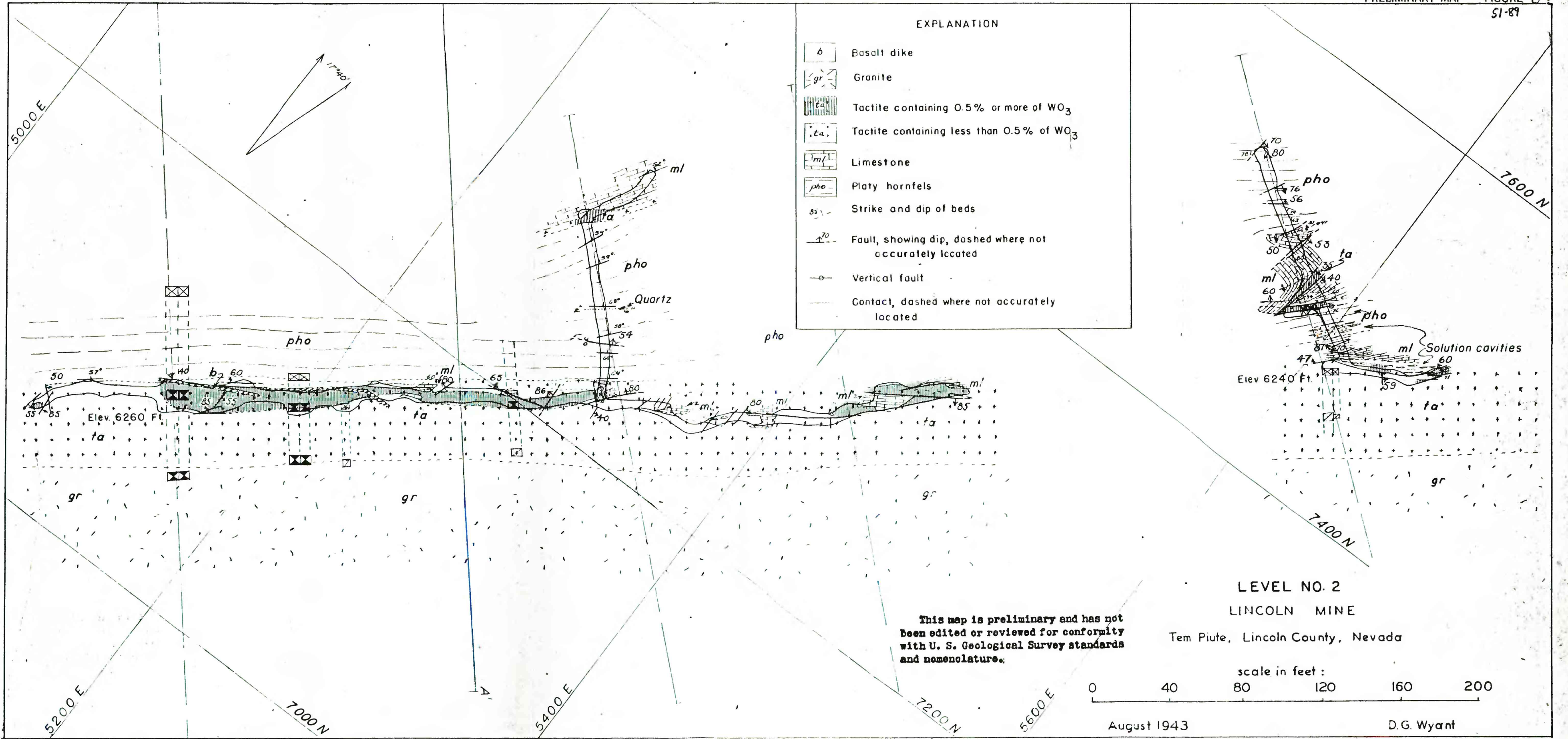
TUNGSTEN DEPOSITS IN THE TEM PIUTE DISTRICT, LINCOLN COUNTY, NEVADA
