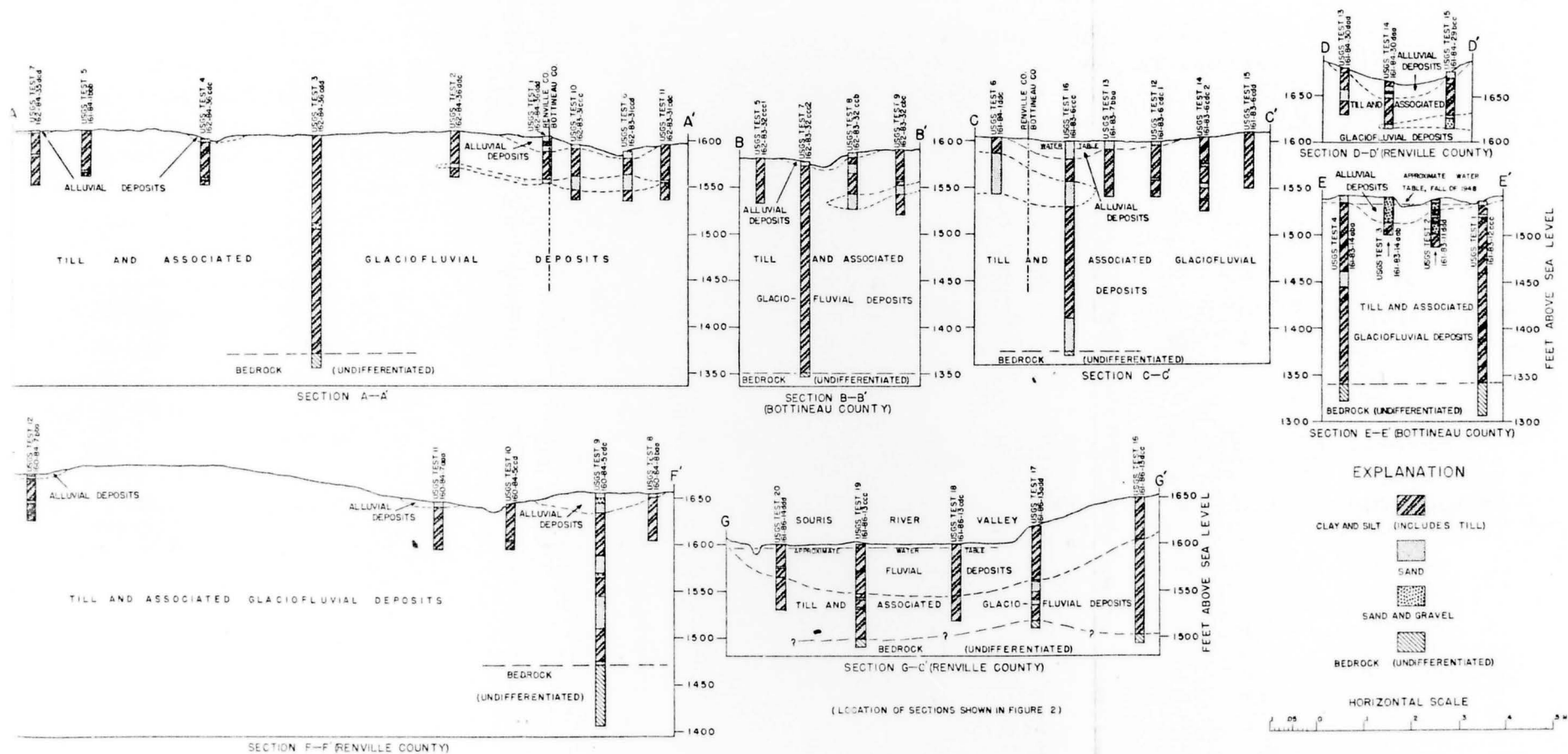
FIGURE 3—GEOLOGIC SECTIONS IN THE MOHALL AREA AND IN THE SOURIS RIVER VALLEY WEST OF MOHALL
