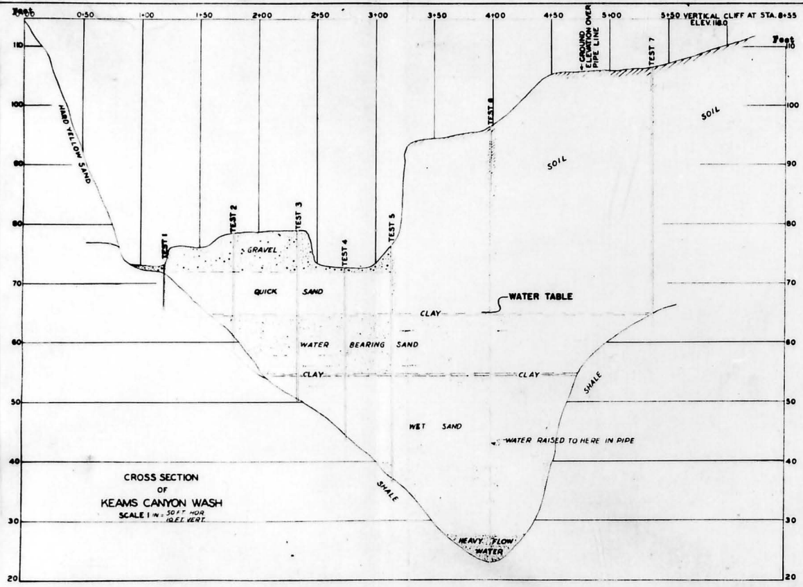
Figure 2. Cross-section of alluvial fill in wash at Keams Canyon, prepared by engineers of Office of Indian Affairs in 1930.
