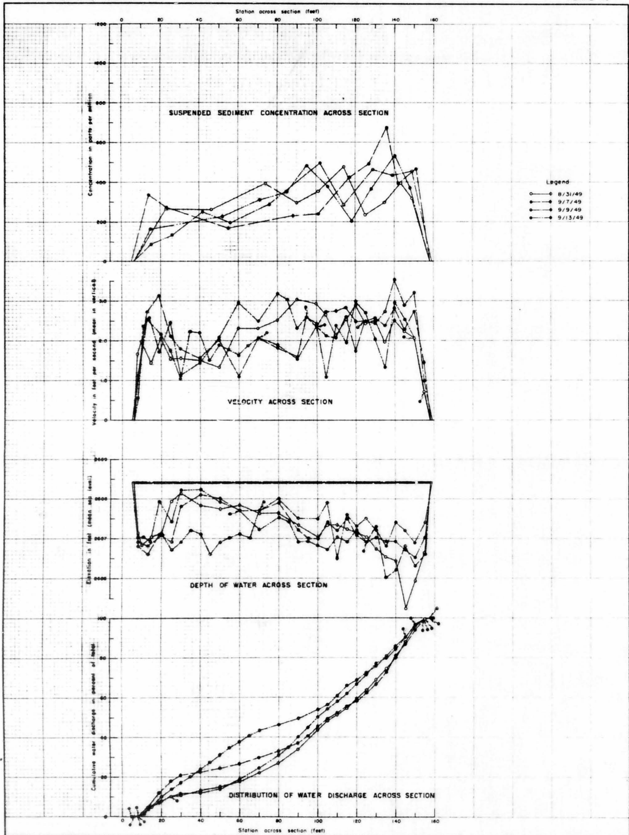
DISCHARGE CHARACTERISTICS OF SECTION E ON THE MIDDLE LOUP RIVER AT DUNNING, NEBRASKA
