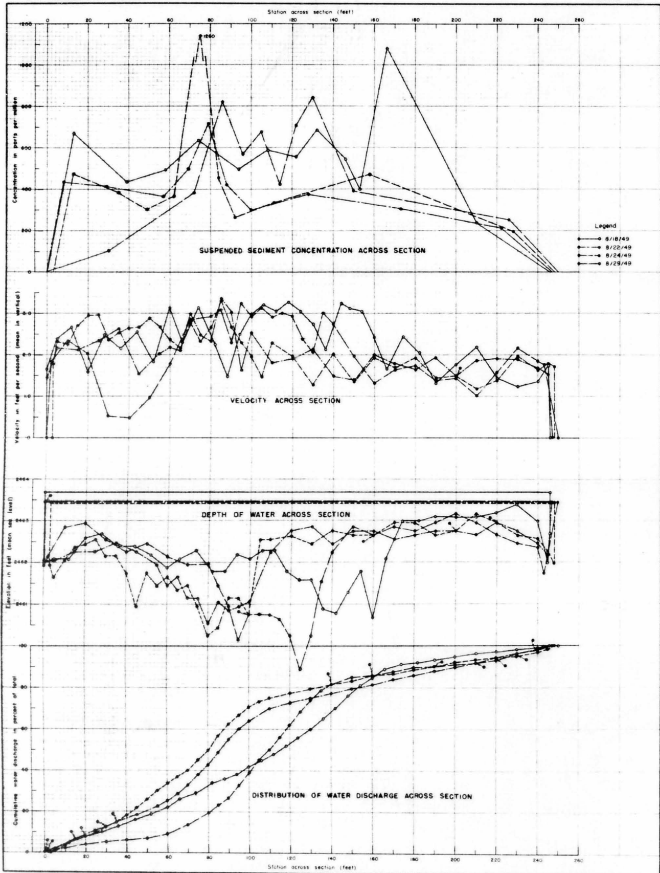
DISCHARGE CHARACTERISTICS OF SECTION G ON THE MIDDLE LOUP RIVER NEAR MILBURN, NEBRASKA
