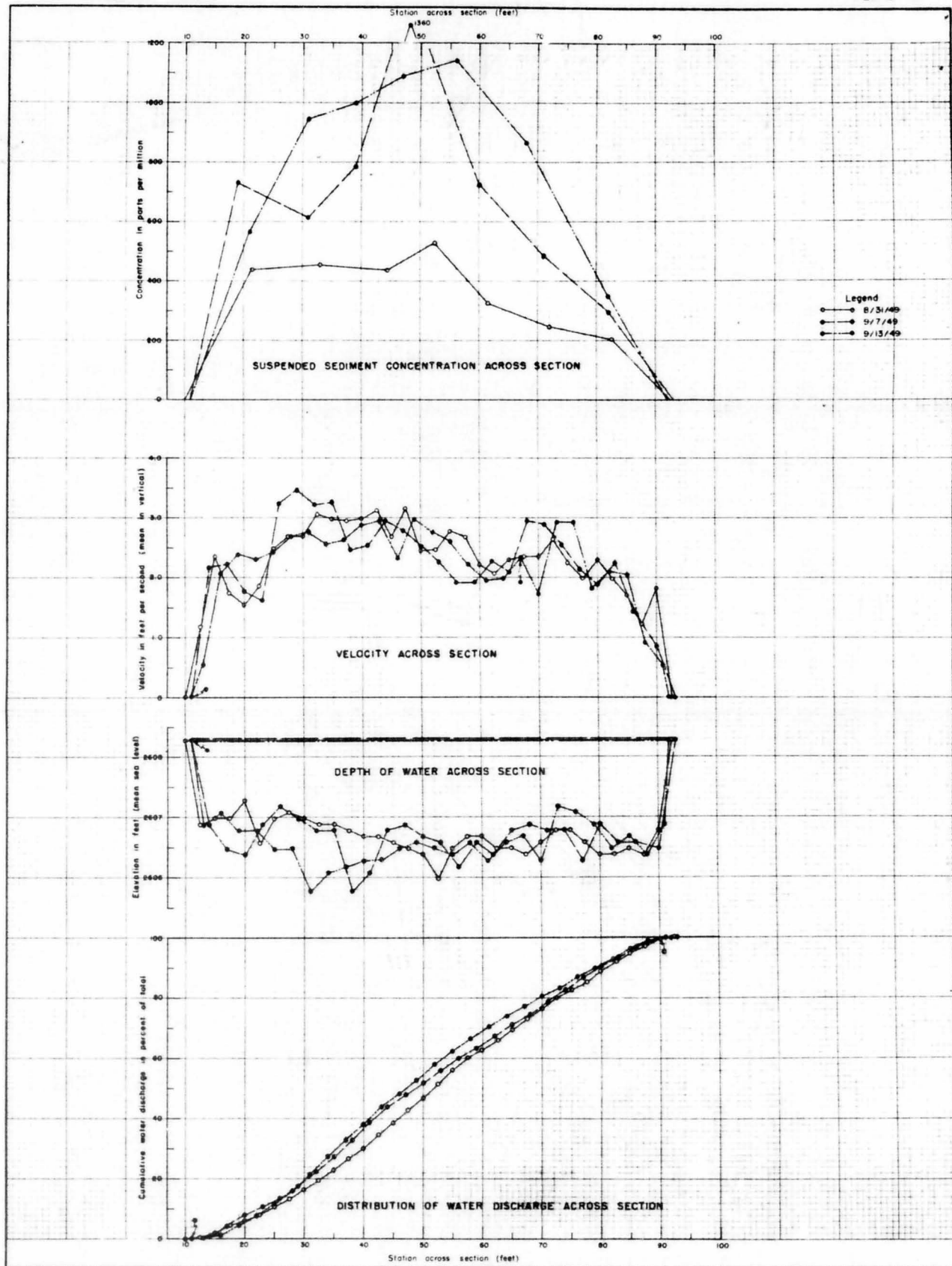
DISCHARGE CHARACTERISTICS OF SECTION H ON THE DISMAL RIVER AT DUNNING, NEBRASKA
