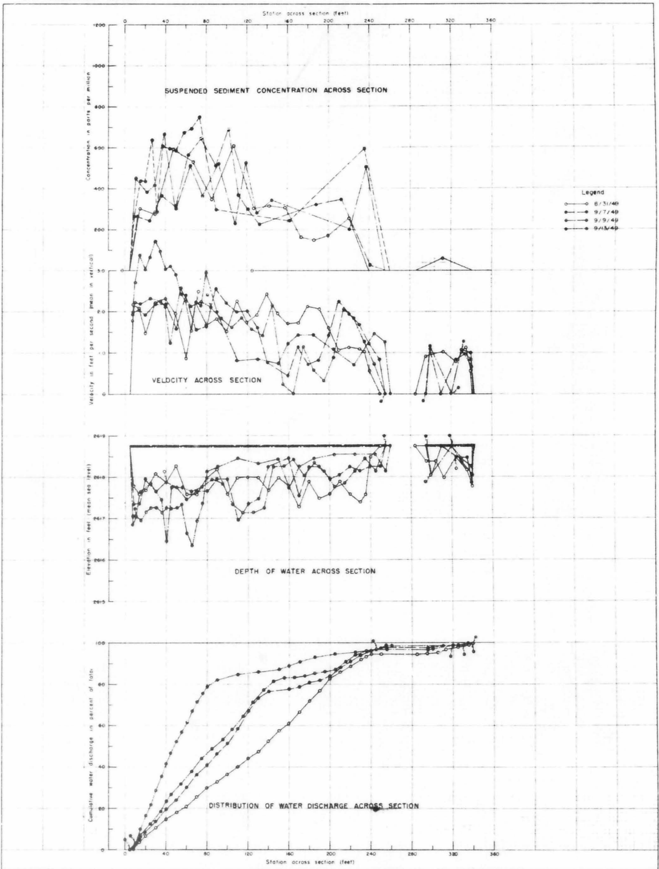
DISCHARGE CHARACTERISTICS OF SECTION A ON THE MIDDLE LOUP RIVER NEAR DUNNING, NEBRASKA
