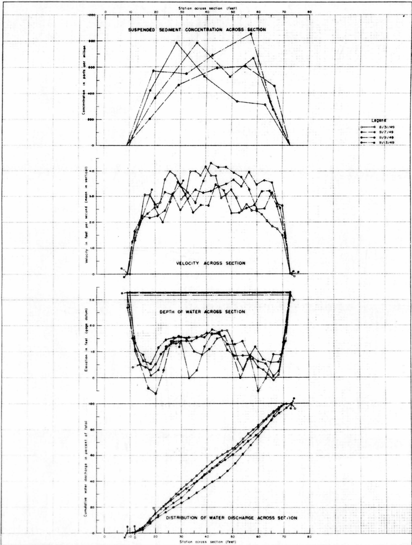
DISCHARGE CHARACTERISTICS OF SECTION B ON THE MIDDLE LOUP RIVER AT DUNNING, NEBRASKA
