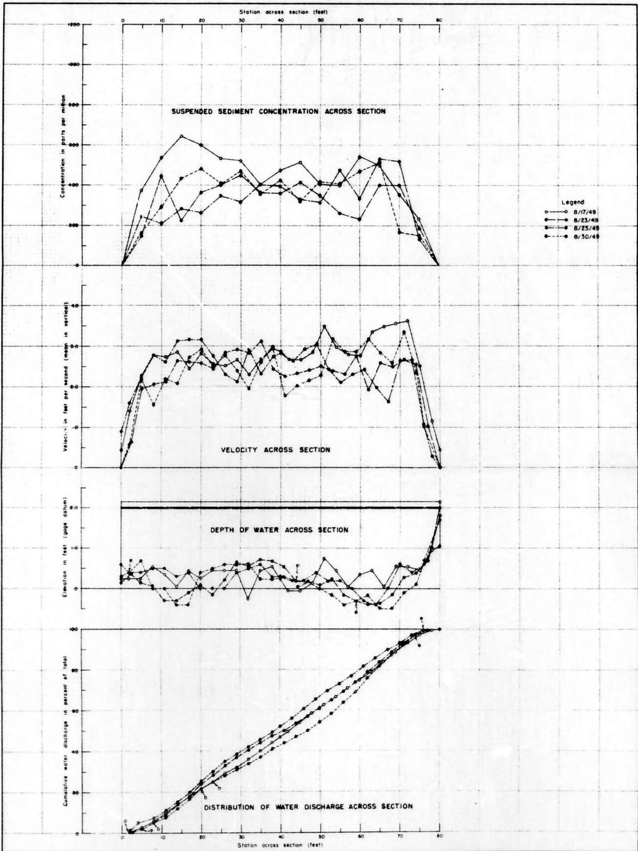
DISCHARGE CHARACTERISTICS OF SECTION C ON THE MIDDLE LOUP RIVER AT DUNNING, NEBRASKA
