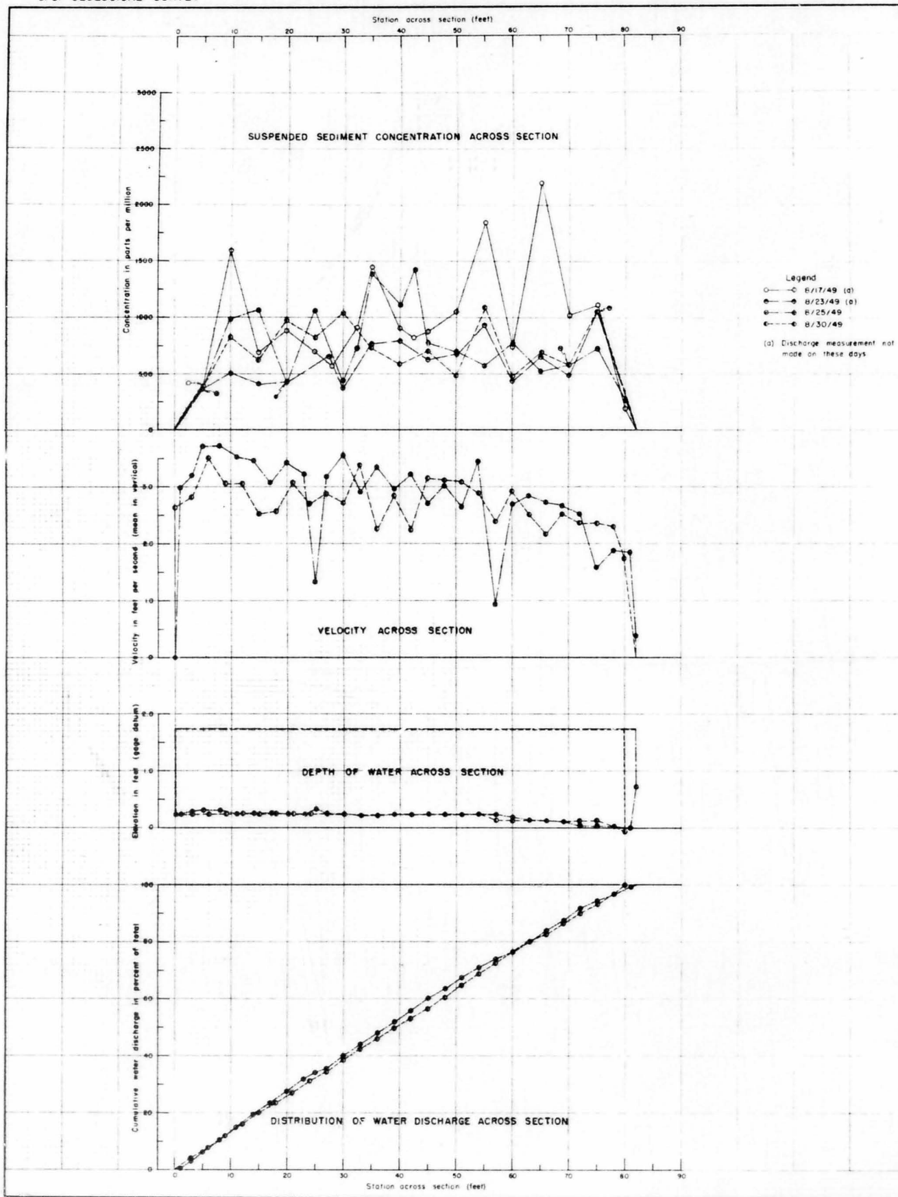
DISCHARGE CHARACTERISTICS OF SECTION D ON THE MIDDLE LOUP RIVER AT DUNNING, NEBRASKA
