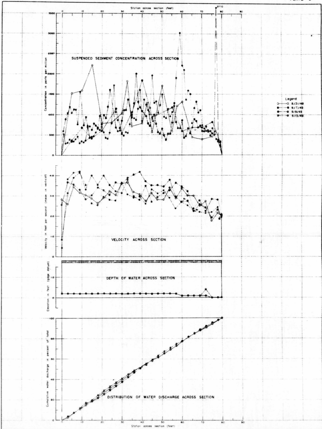
DISCHARGE CHARACTERISTICS OF SECTION D ON THE MIDDLE LOUIP RIVER AT DUNNING, NEBRASKA
