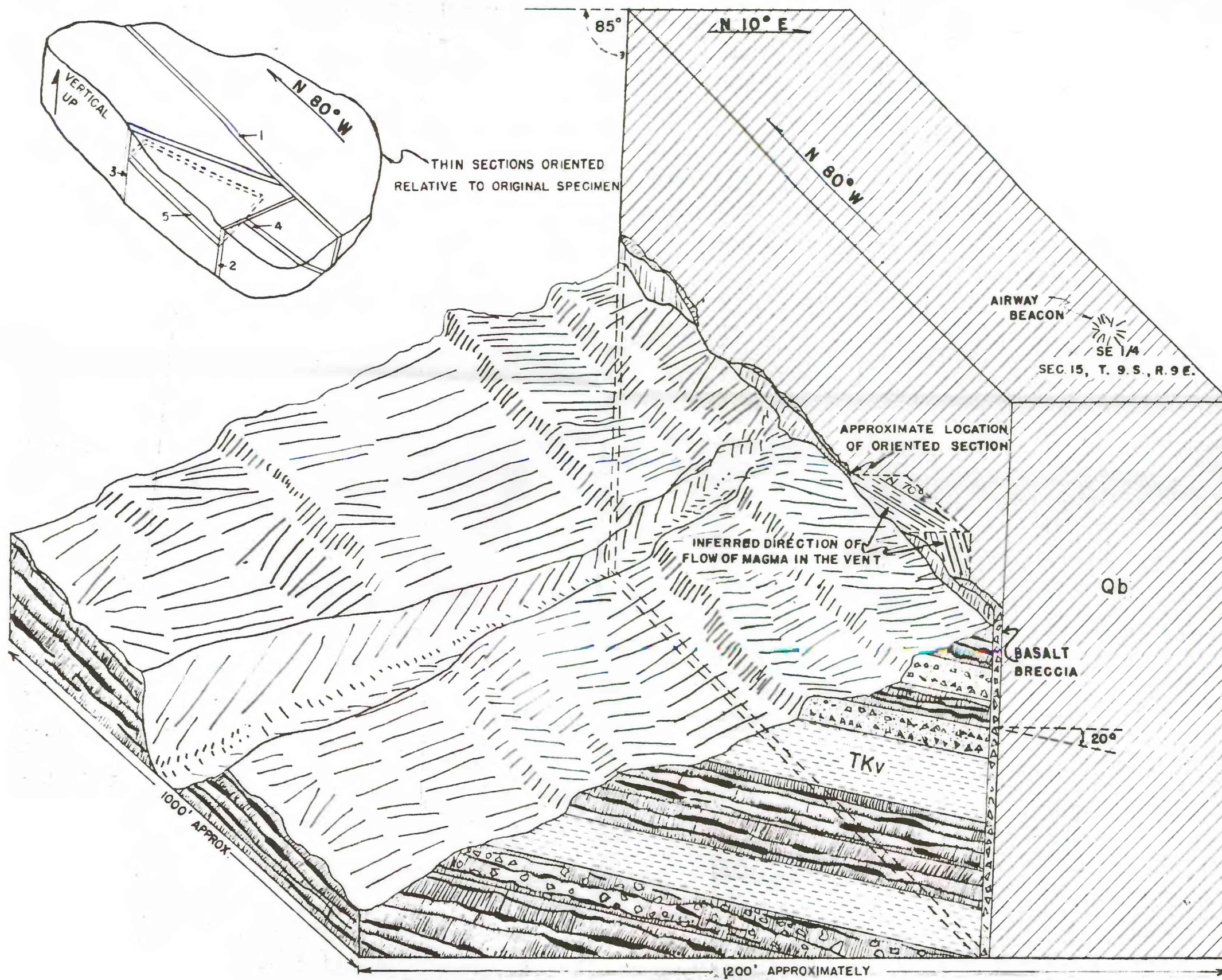
FIGURE 5. BLOCK DIAGRAM OF PICACHO PEAK SHOWING INFERRED RELATIONSHIPS. SECTION ACROSS FLOWS IS GENERALIZED. SEE FIGURE 1 FOR EXPLANATION OF SYMBOLS
