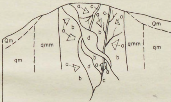
Figure 4.- Sketch illustrating four ages of silica.
