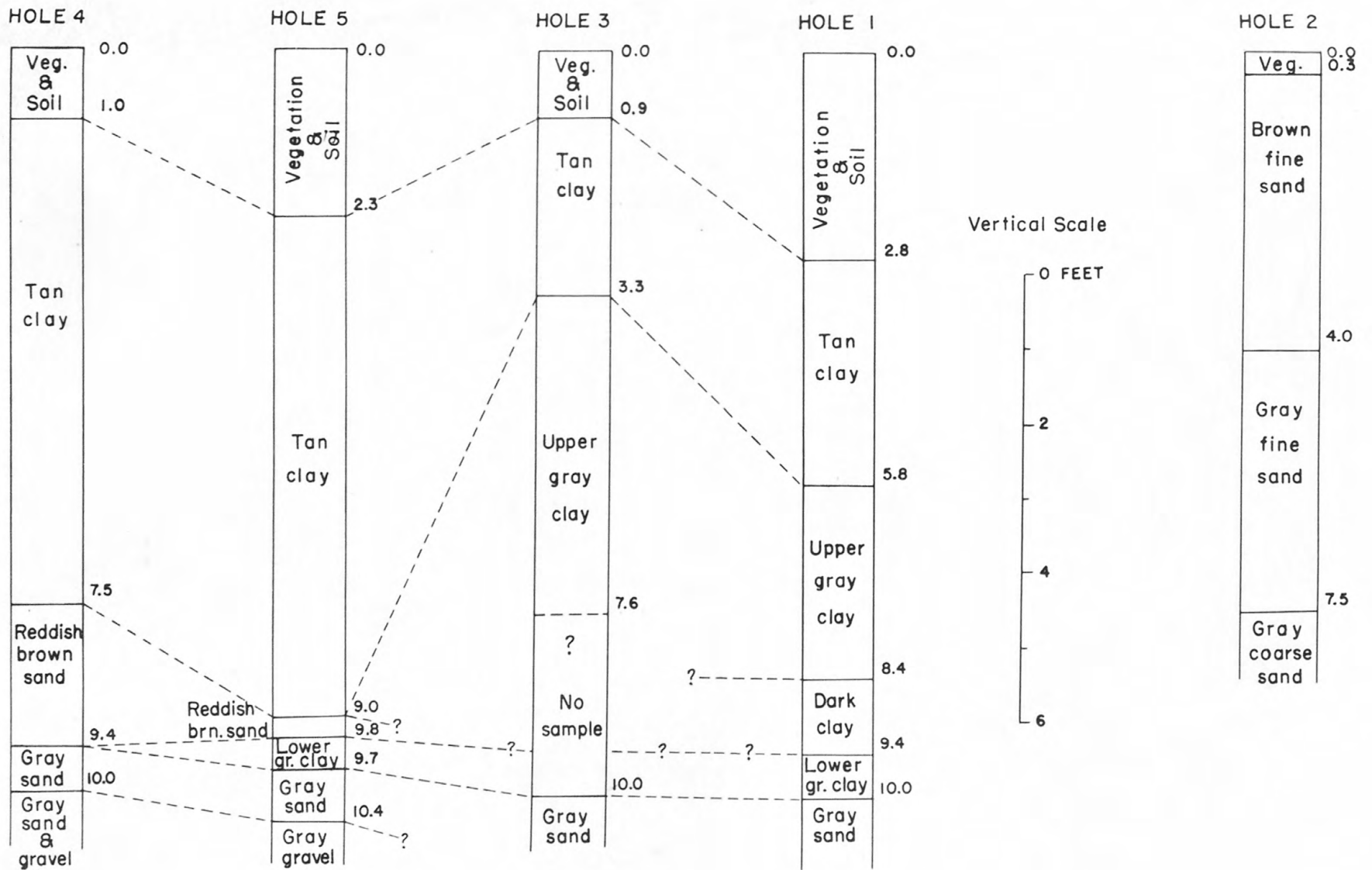
Figure 3: Logs of auger holes in clay deposit near Nenana, Alaska (See figure 2 for locations, and text for explanation of lower part of Hole 3.)
