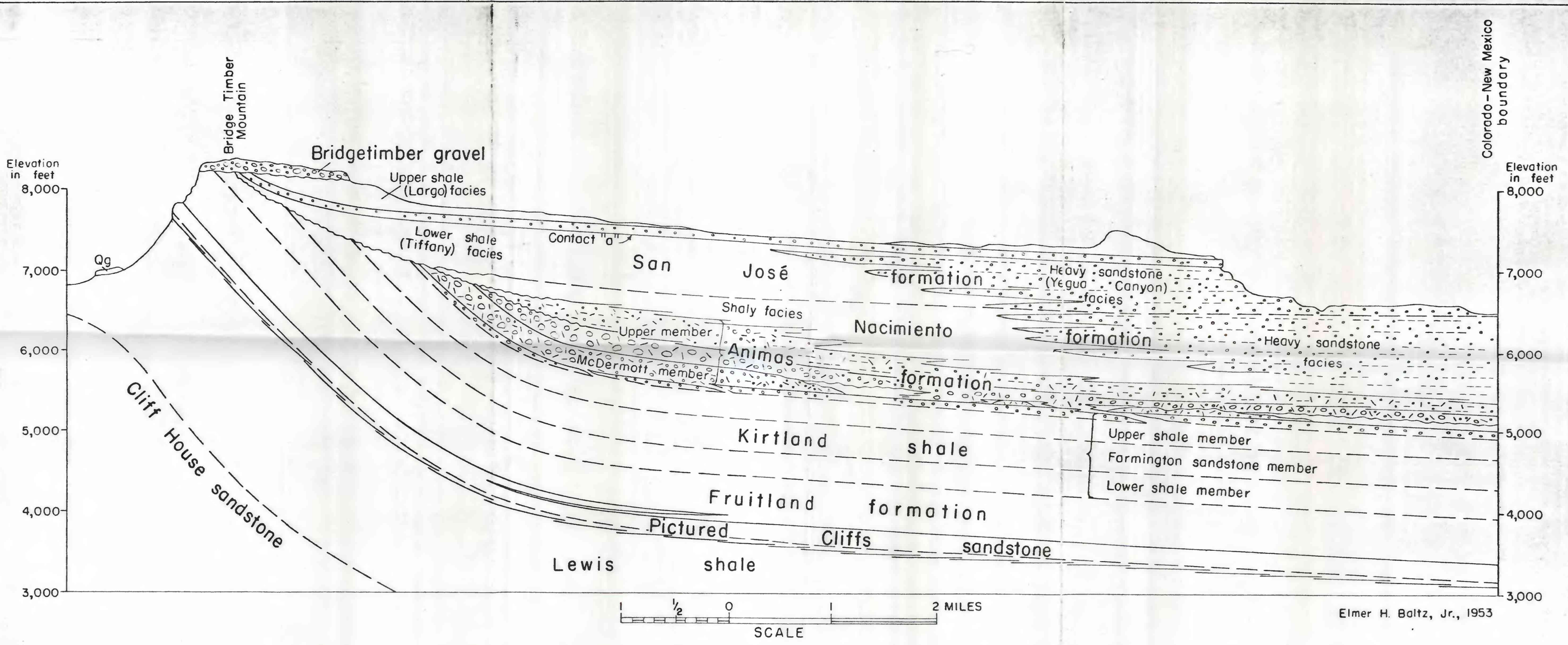
Figure 6. Diagram showing stratigraphic relationships of Upper Cretaceous and lower Tertiary rocks in the Bridge Timber Mountain area, La Plata County, Colorado.
