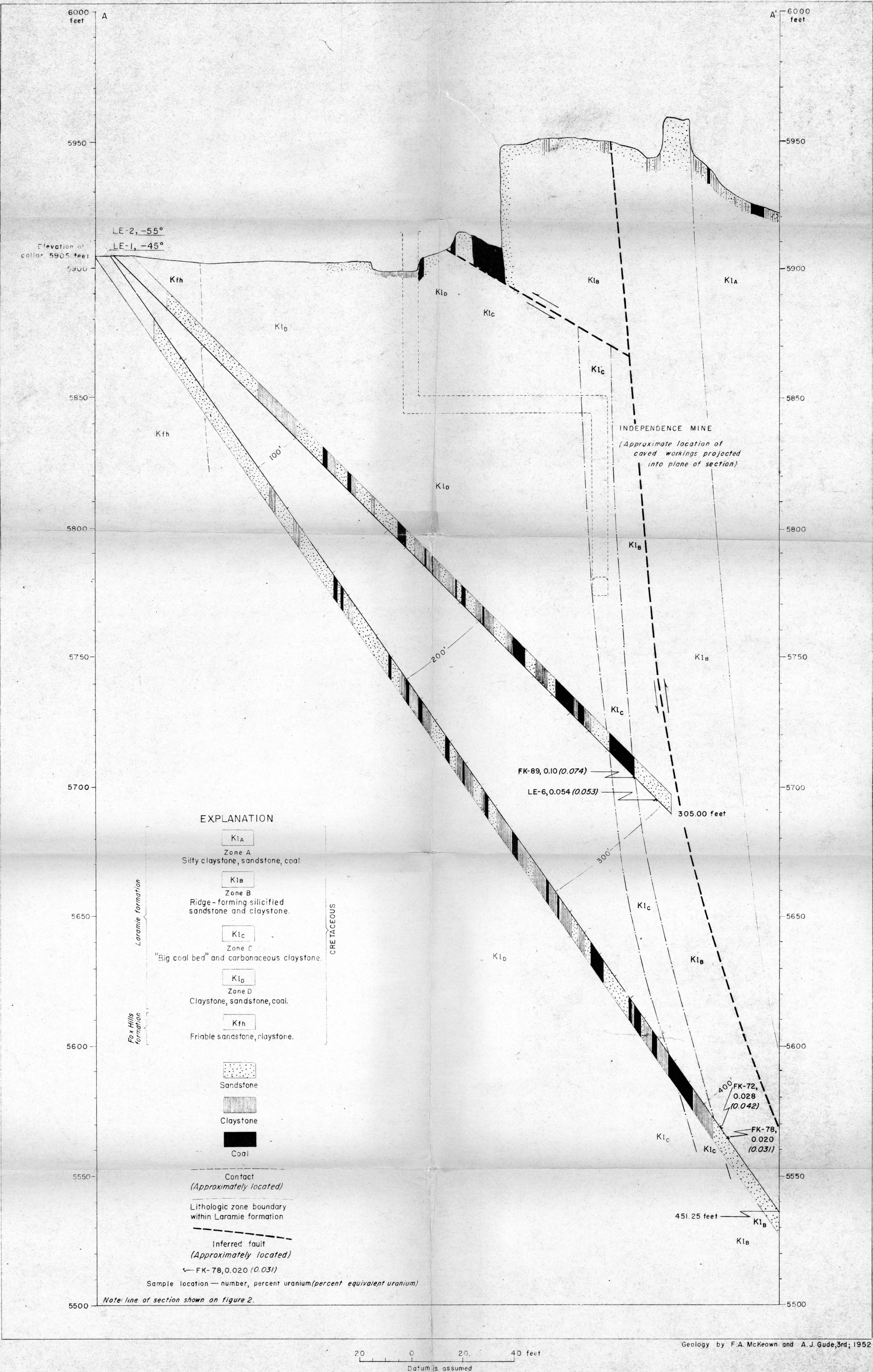
FIGURE 3.--SECTION THROUGH DIAMOND DRILL HOLES LE-1 AND LE-2, OLD LEYDEN COAL MINE, JEFFERSON COUNTY, COLORADO
