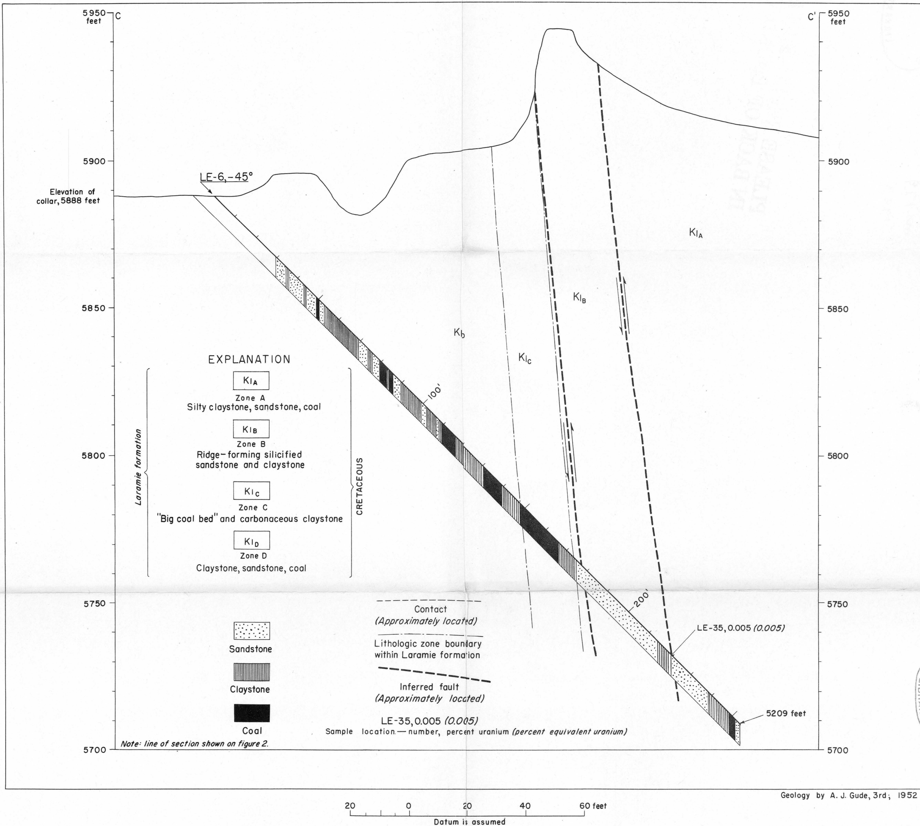
FIGURE 5.--SECTION THROUGH DIAMOND DRILL HOLE LE-6, OLD LEYDEN COAL MINE, JEFFERSON COUNTY, COLORADO
