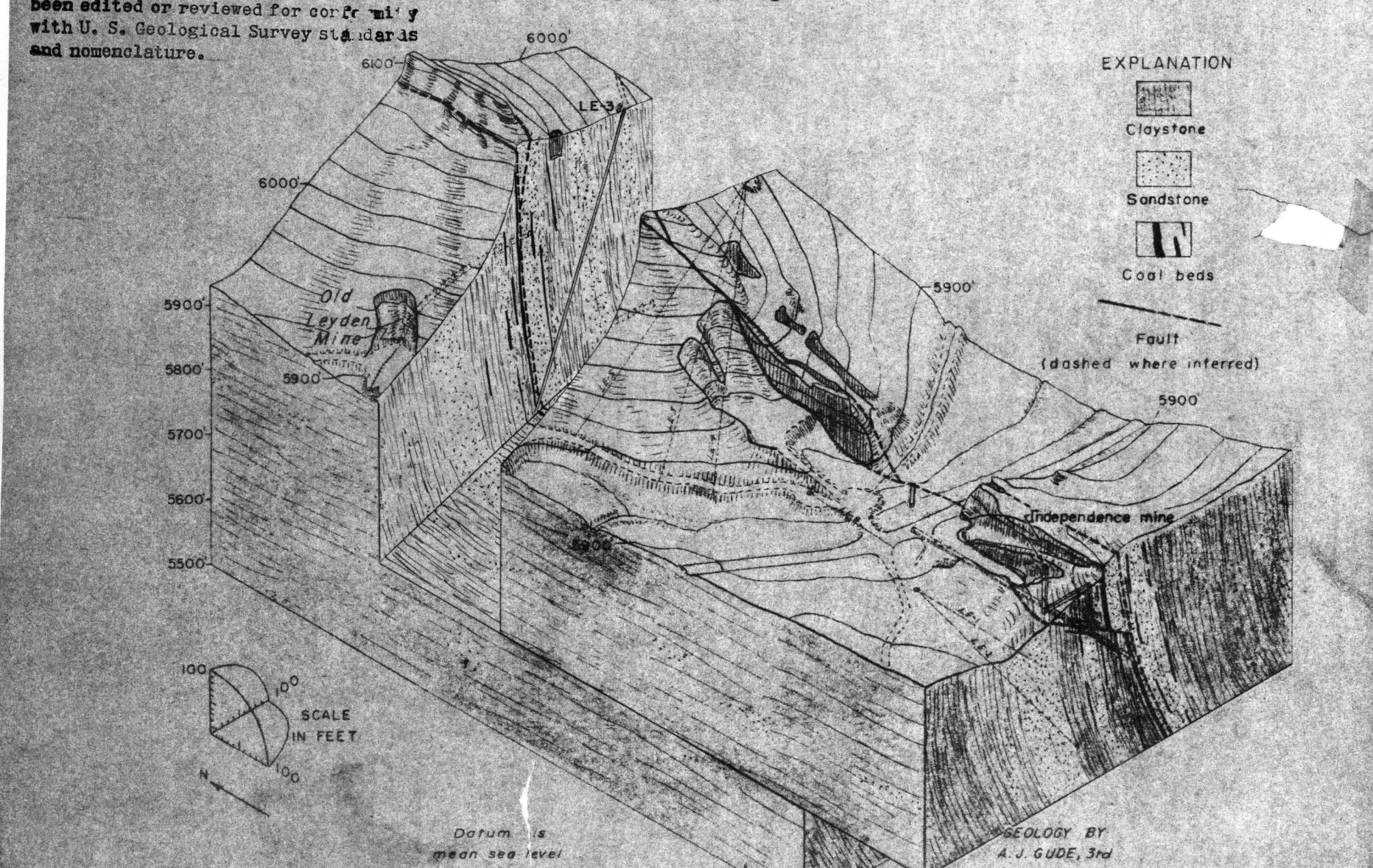
Figure 8.-- BLOCK DIAGRAM SHOWING LOCATION OF HOLE LE-3
