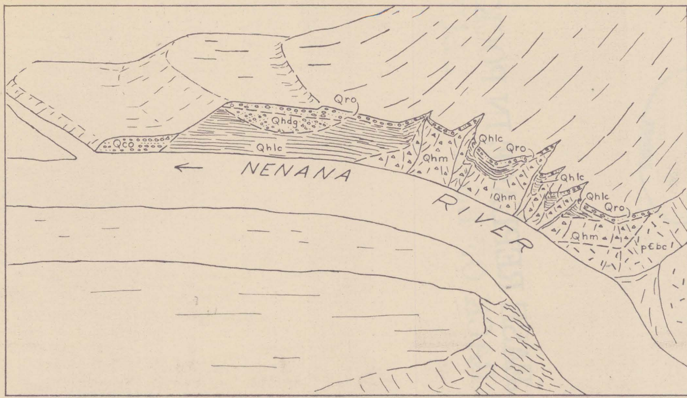
Figure 10.--Field sketch of geologic conditions on northeast bank of the Nenana River one mile north of McKinley Park station. Qco, outwash of the Carlo re-advance; Qro, outwash of the Riley Creek glaciation; Qhdg, delta gravel in Glacial Lake Moody; Qhlc, lake clay of Glacial Lake Moody; Qhm, till of the Healy glaciation; pEbc, Birch Creek schist. Geologic contacts shown by dashed lines.
