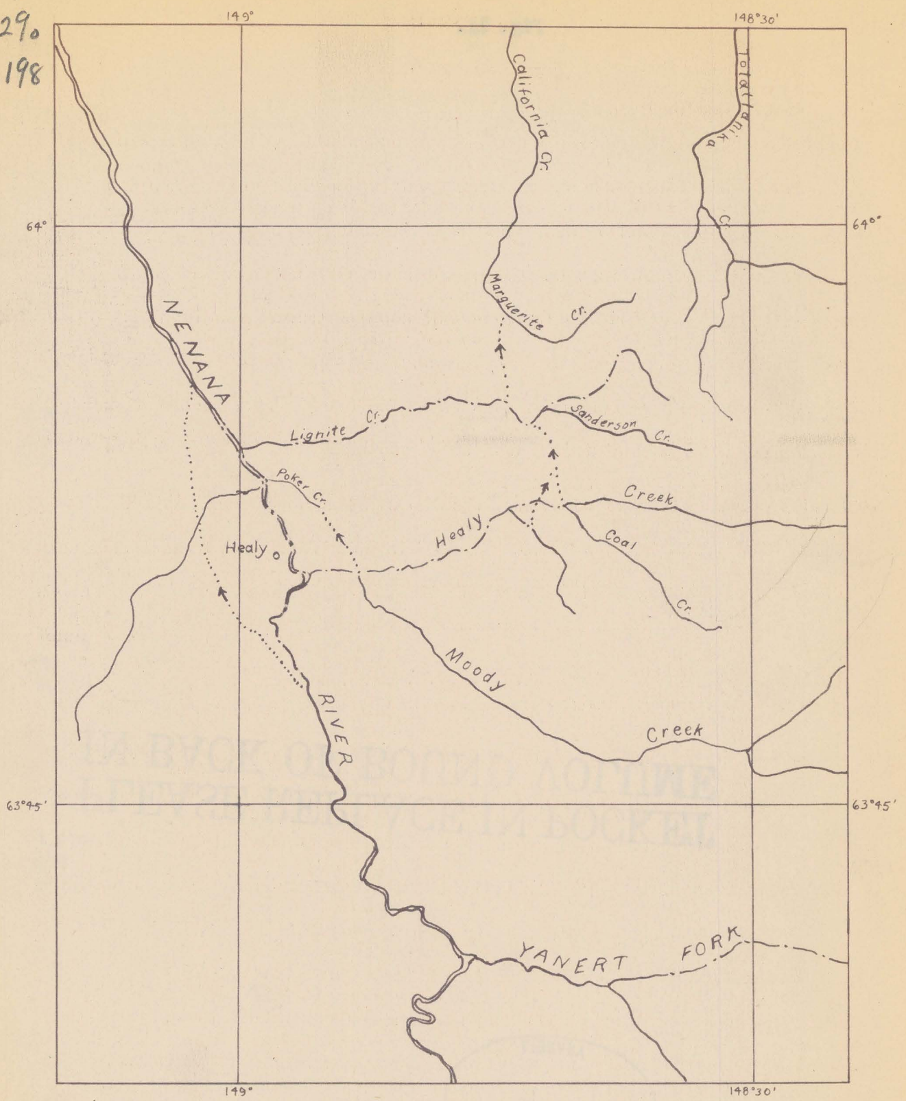
Figure 11.--Drainage changes on tributaries of the Nenana River from the beginning of the Dry Creek to the end of the Healy glaciation. Solid lines, stream courses relatively unchanged from the beginning of the Dry Creek glaciation to the present; dash-dot lines, stream courses developed since the Dry Creek; dotted lines, stream courses abandoned since the Dry Creek glaciation.
