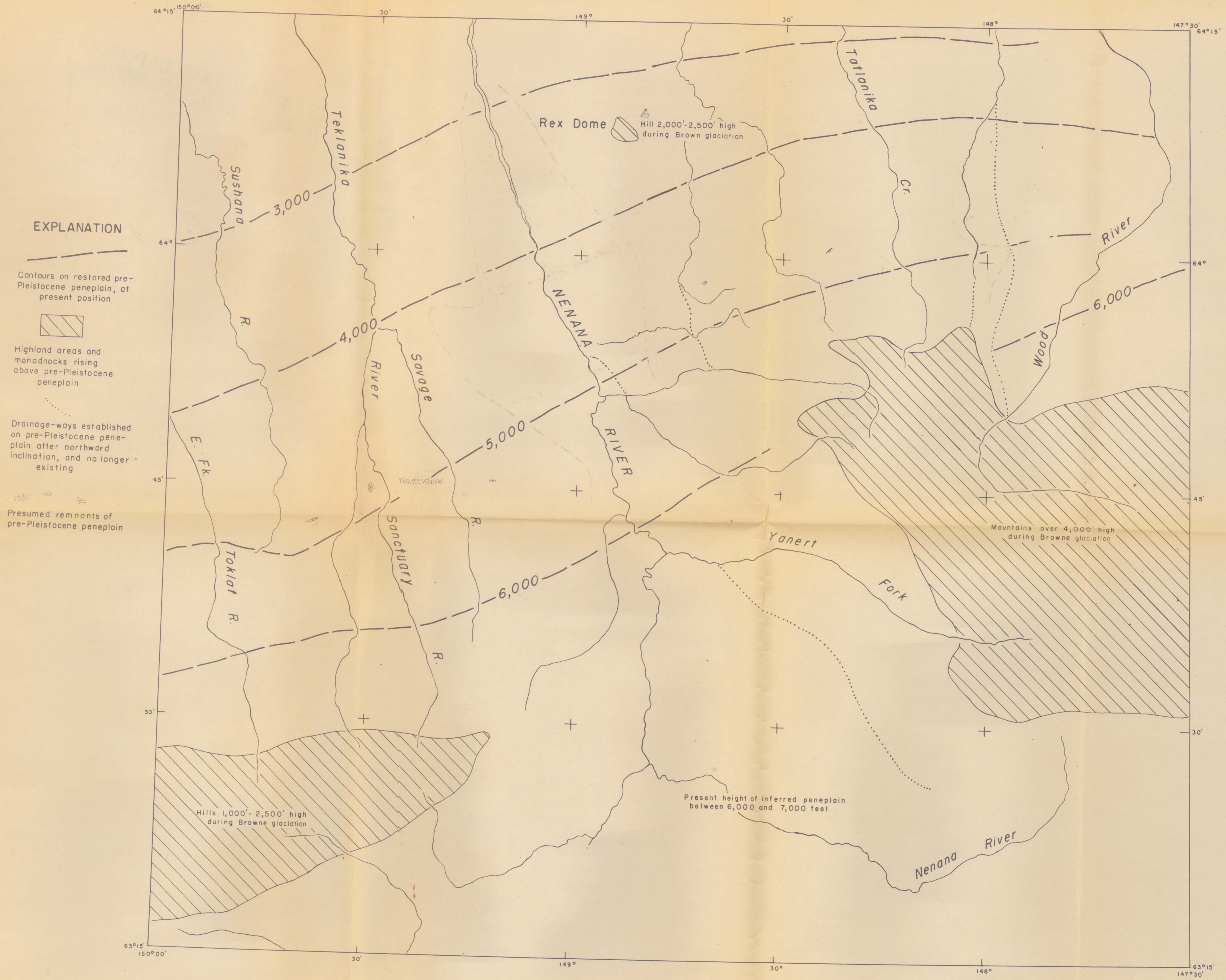
Fig. 4. Reconstructed geography of the Alaska Range prior to the Browne Glaciation
