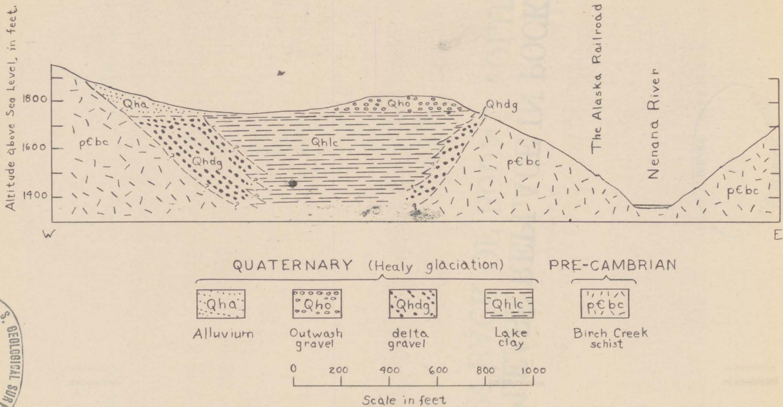
Figure 7.—Geologic cross-section of the floor of the glacial Nenana River gorge at mile 35 1/2 on the Alaska Railroad, showing buried lake deposits west of the river. Topography from Alaska Railroad bridge engineer's map, scale 1:1,800.
