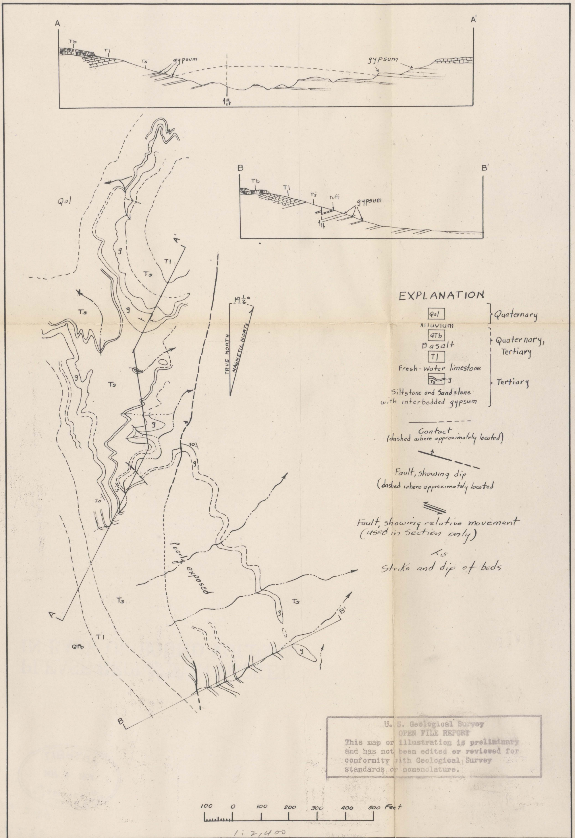
FIG. 13.—GEOLOGIC MAP AND SECTIONS OF THE GYPSUM AREA, SAN CARLOS INDIAN RESERVATION
