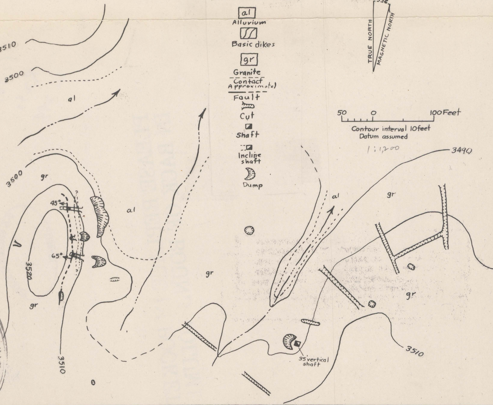
FIG. 6.—GEOLOGIC SKETCH MAP OF THE PEACOCK COPPER WORKINGS, SAN CARLOS INDIAN RESERVATION
