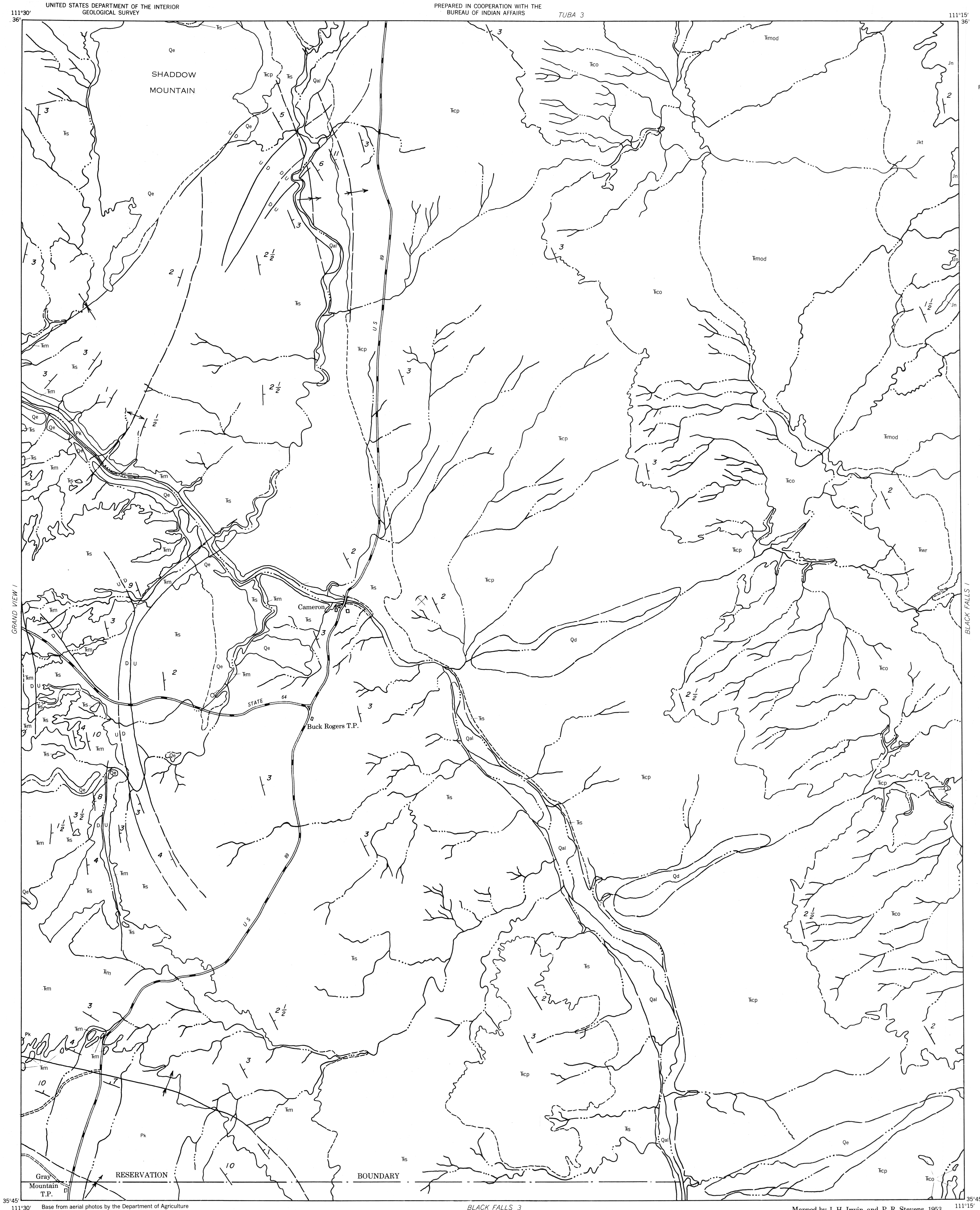
PRELIMINARY GEOLOGIC MAP OF THE BLACK FALLS 2 QUADRANGLE, ARIZONA
