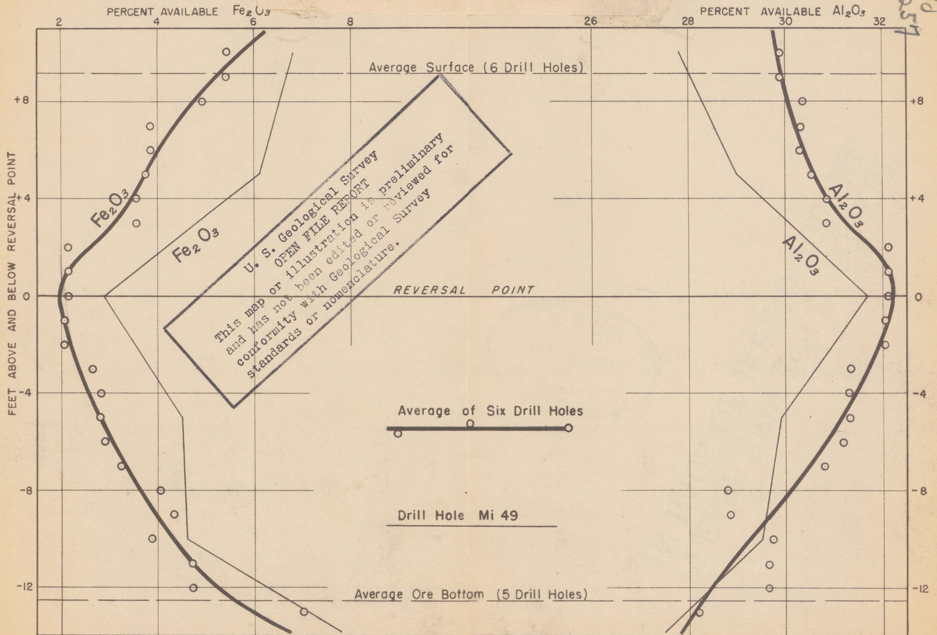
Fig. 2 Variation of available \text{Fe}_2\text{O}_3 and \text{Al}_2\text{O}_3 with depth for the ore portion of the Excelsior residual basaltic clay blanket.
