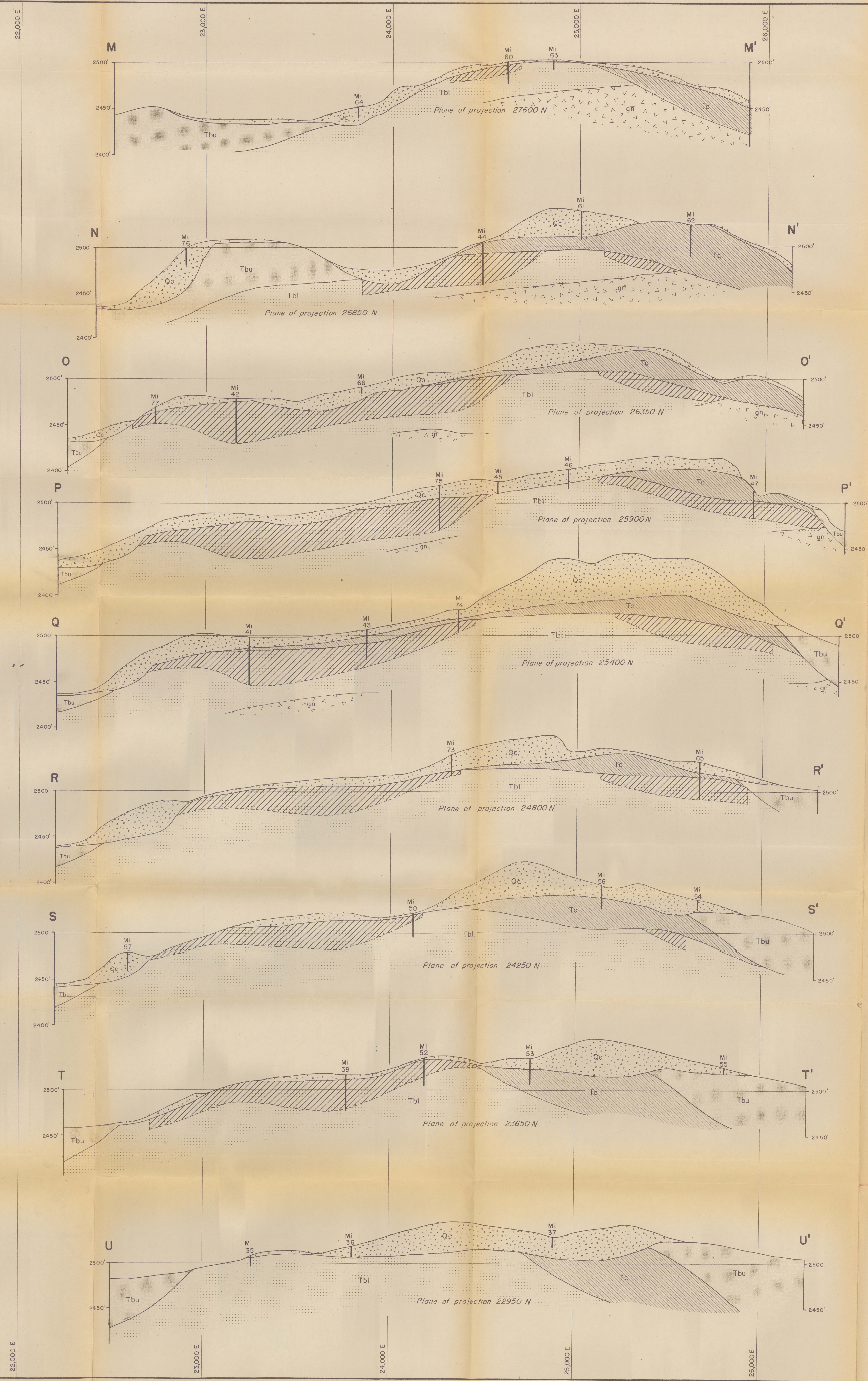
EAST-WEST GEOLOGIC SECTIONS OF AREA II, EXCELSIOR HIGH-ALUMINA CLAY DEPOSIT, SPOKANE COUNTY, WASHINGTON
