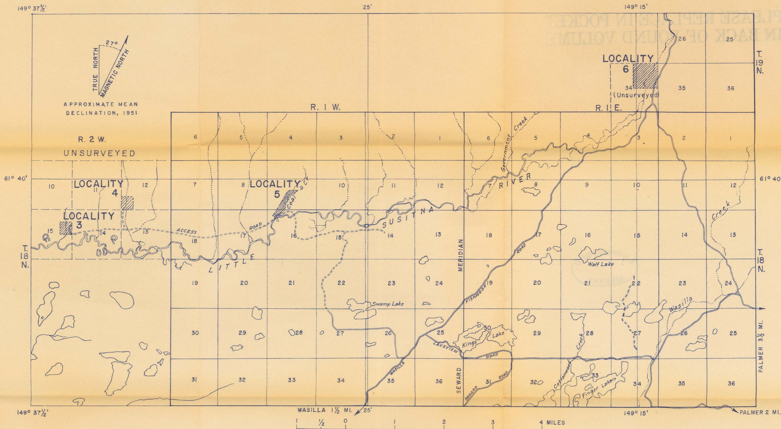
INDEX MAP SHOWING AREAS EXPLORED BY BULLDOZER AND POWER AUGER IN THE LITTLE SUSITNA DISTRICT, MATANUSKA COAL FIELD, ALASKA
