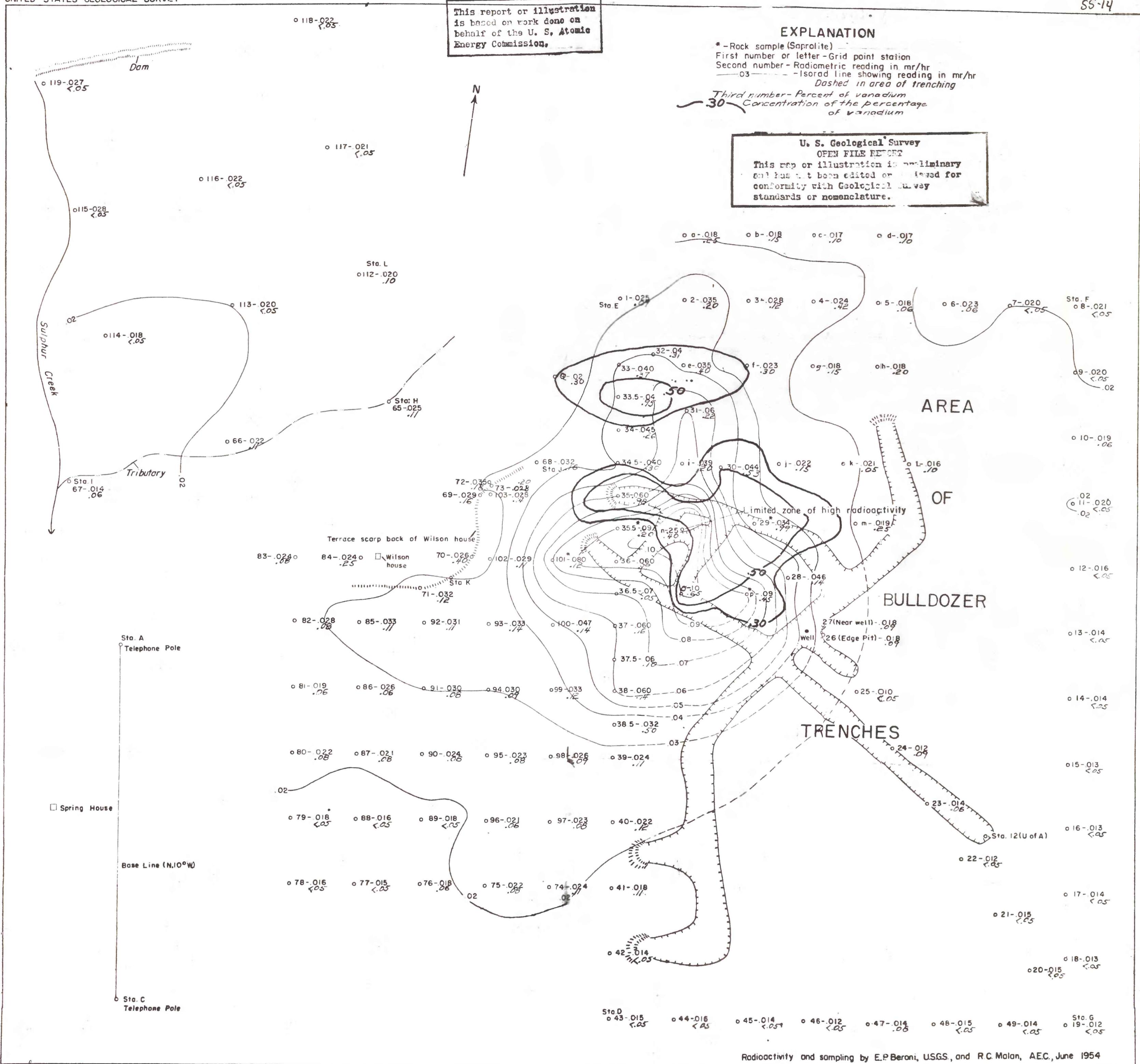
ISORADIATION MAP SHOWING VANADIUM CONCENTRATION IN THE VICINITY OF BULLDOZER TRENCHES, WILSON PROSPECT, GALLAND COUNTY, SA
