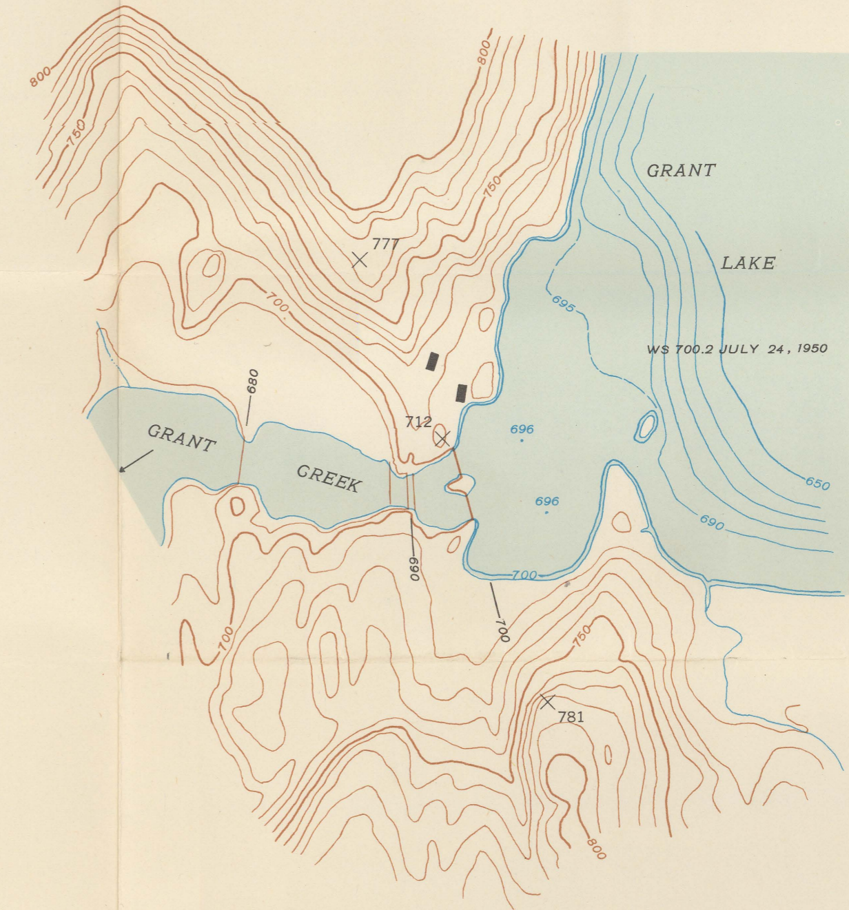
GRANT LAKE DAM SITE
