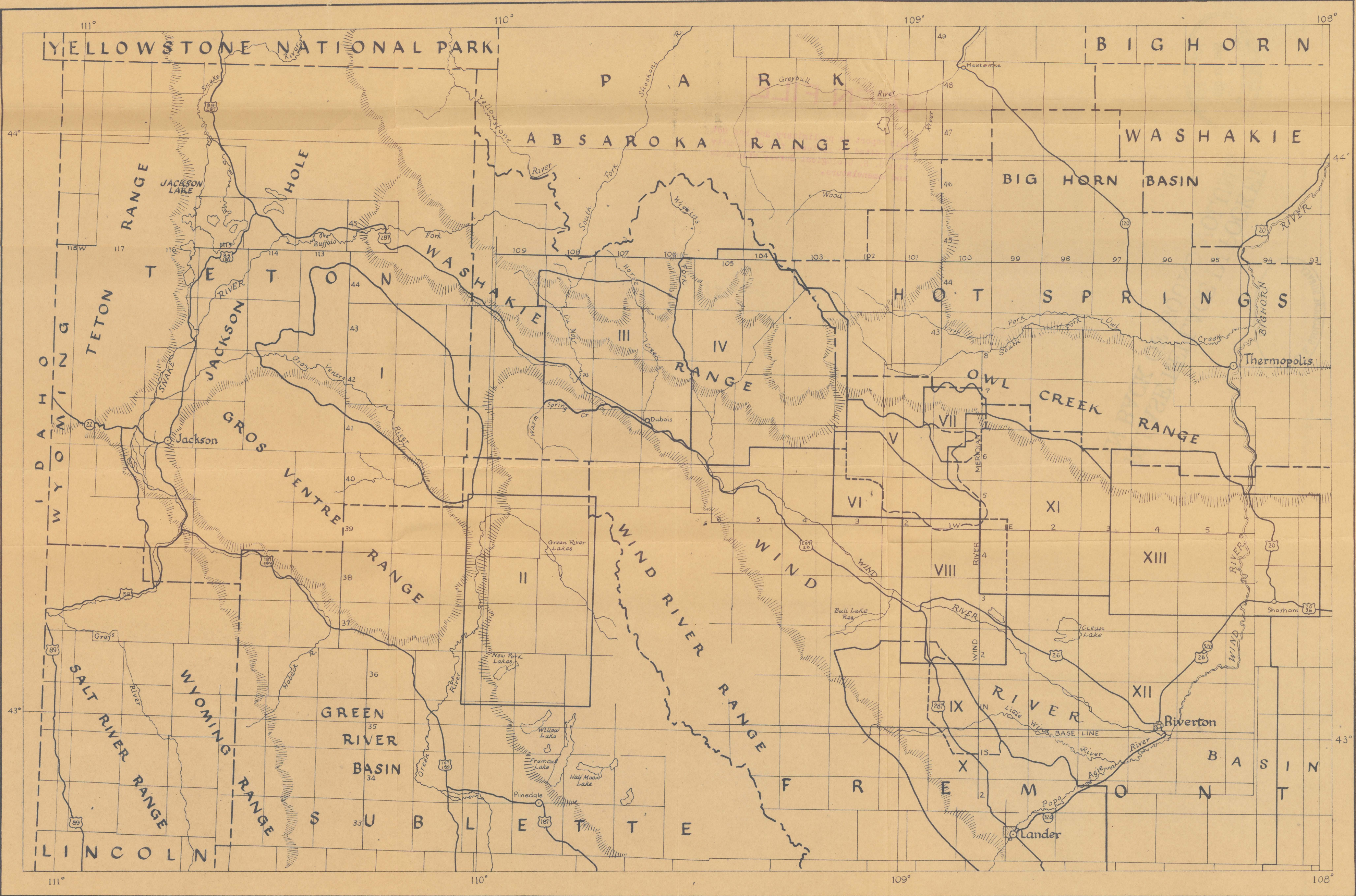
INDEX MAP SHOWING MAJOR PHYSIOGRAPHIC FEATURES AND AREAS OF RECENT GEOLOGIC MAPPING IN WEST-CENTRAL WYOMING
