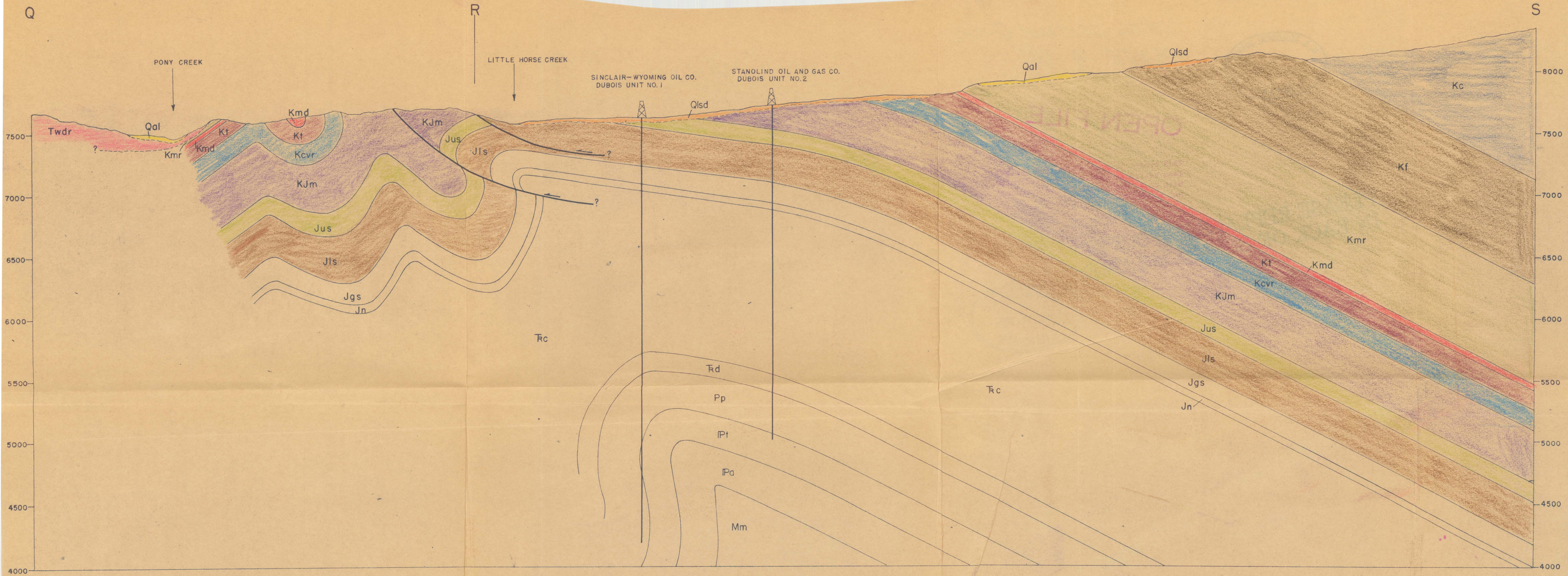
CROSS SECTION Q-R-S
