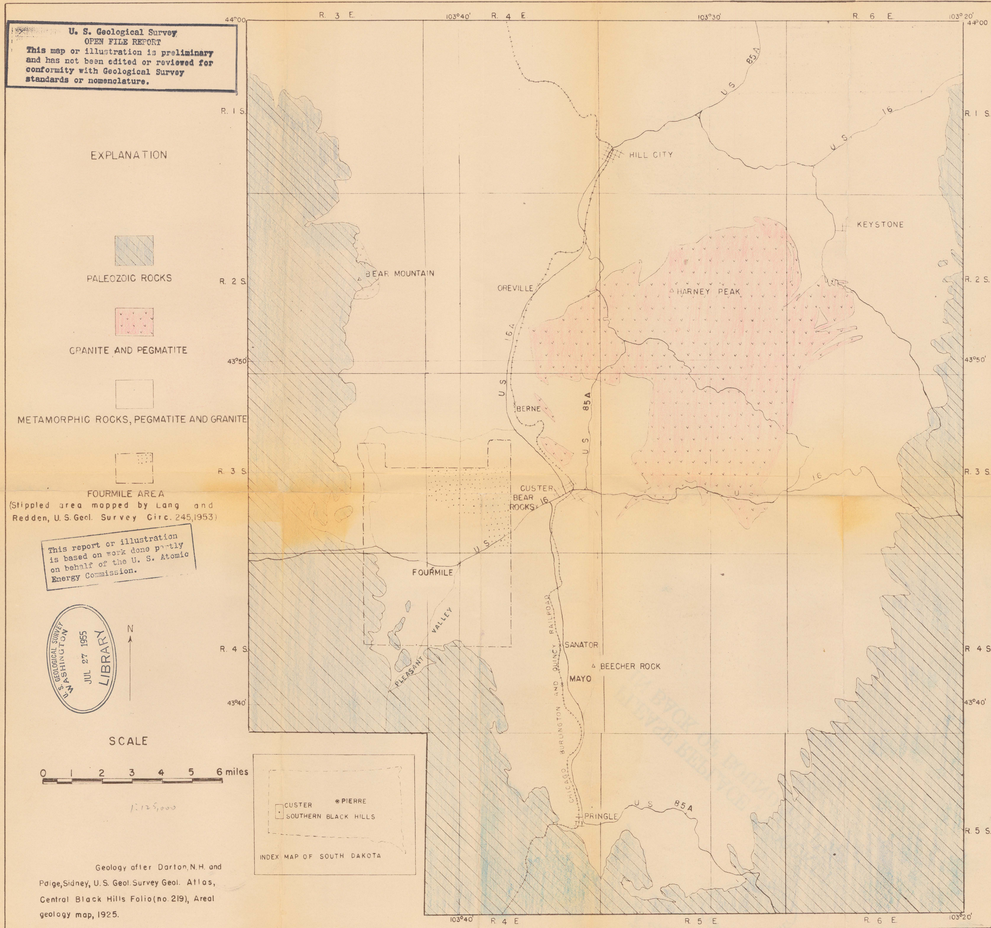
Figure 1.--- GENERALIZED GEOLOGIC MAP OF SOUTHERN BLACK HILLS, SOUTH DAKOTA
