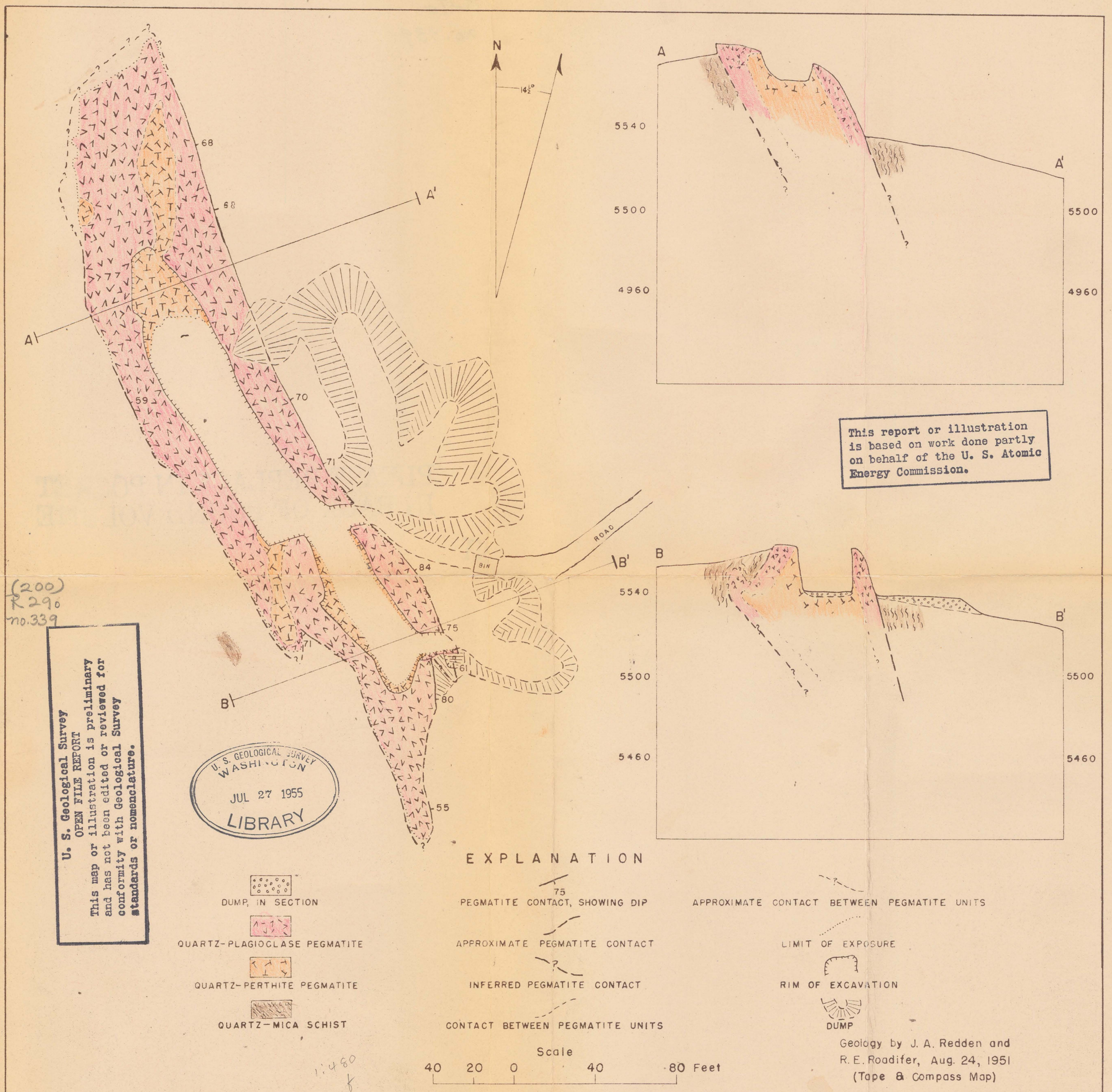
Figure 14.--GEOLOGIC MAP AND SECTIONS, ROCK RIDGE PEGMATITE, CUSTER COUNTY, SOUTH DAKOTA
