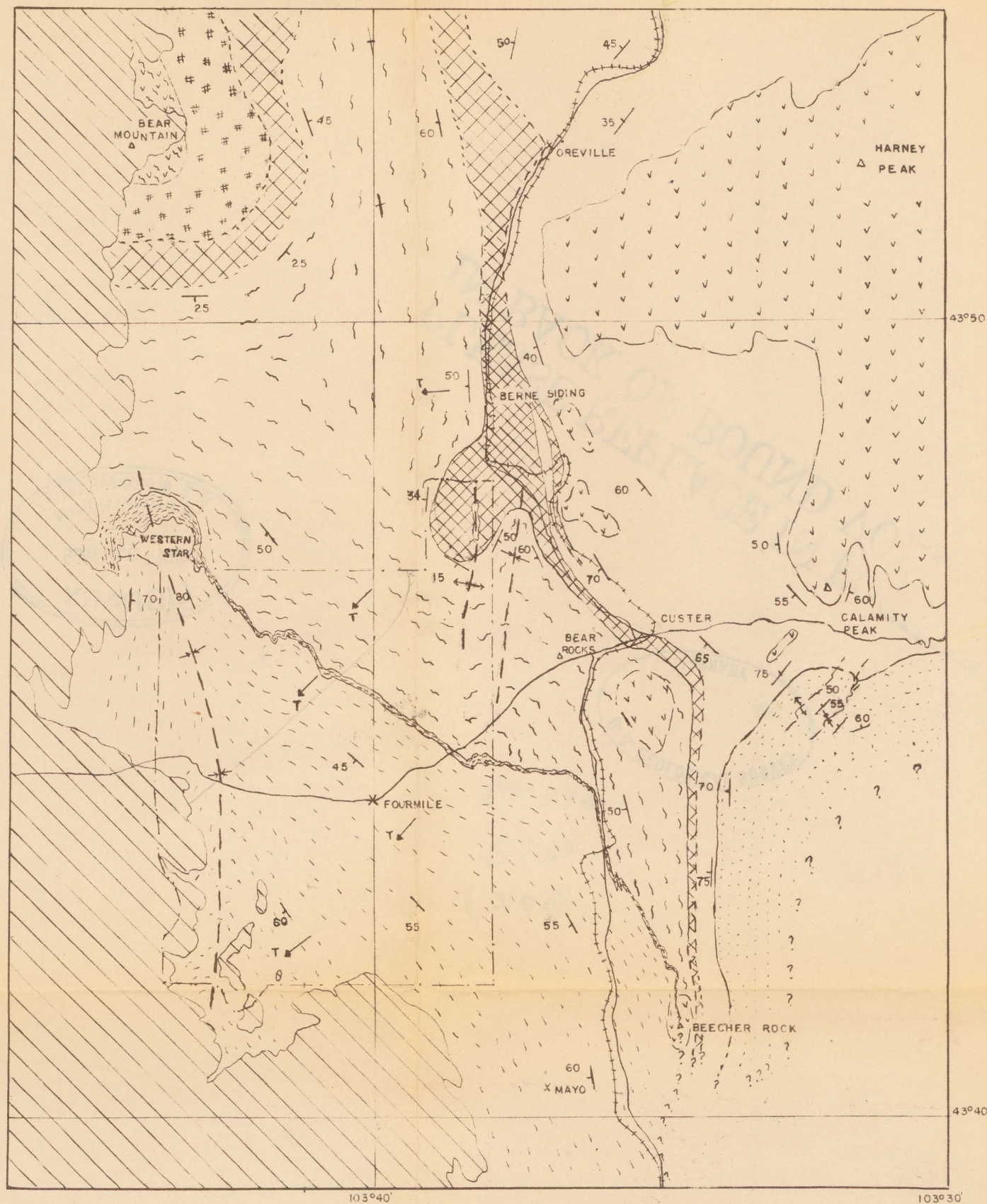
Figure 2...REGIONAL GEOLOGIC SETTING OF THE FOURMILE AREA, CUSTER COUNTY, SOUTH DAKOTA
