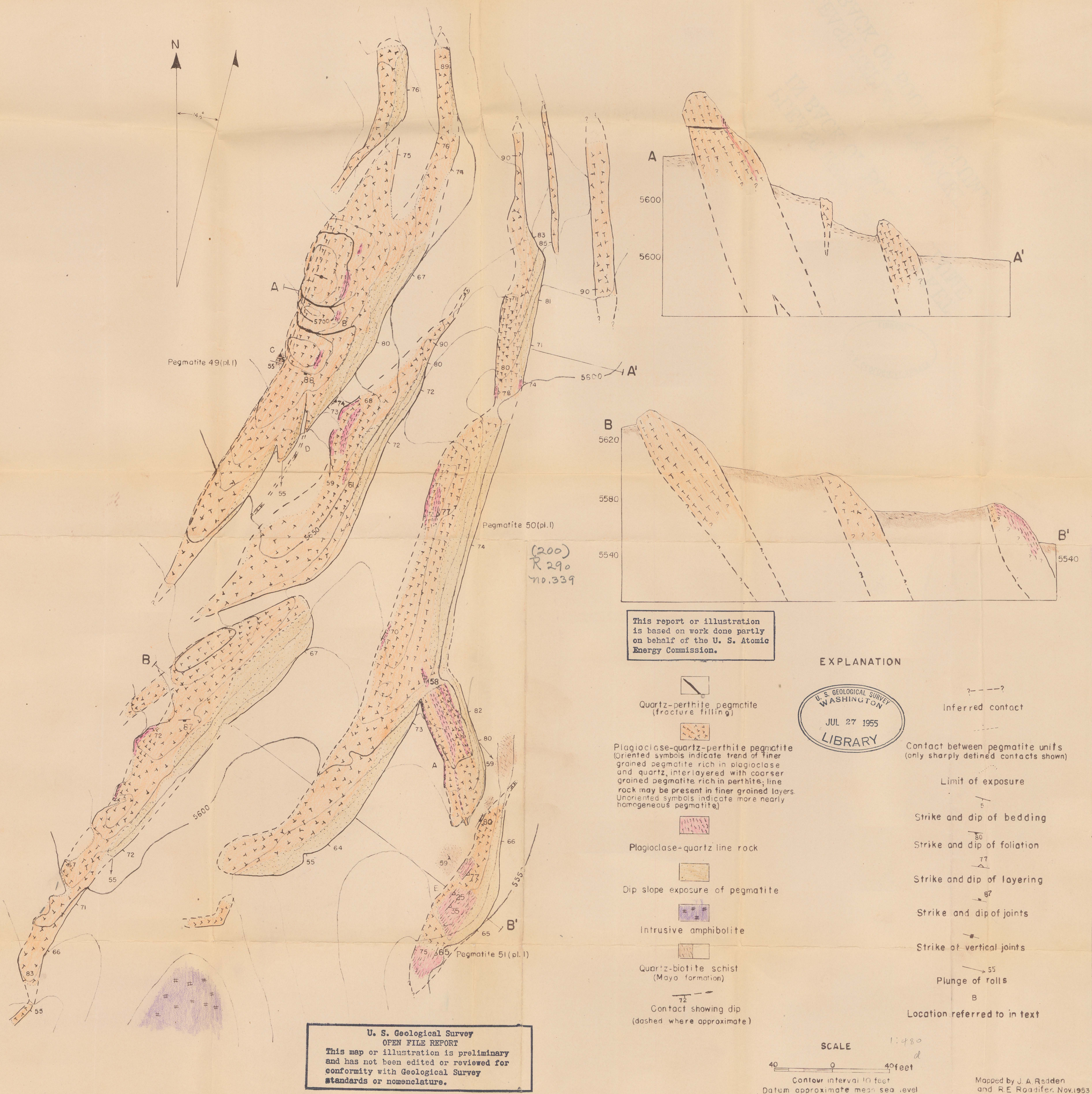
Figure 4.-GEOLOGIC MAP AND SECTIONS OF LAYERED AND HOMOGENEOUS PEGMATITES
