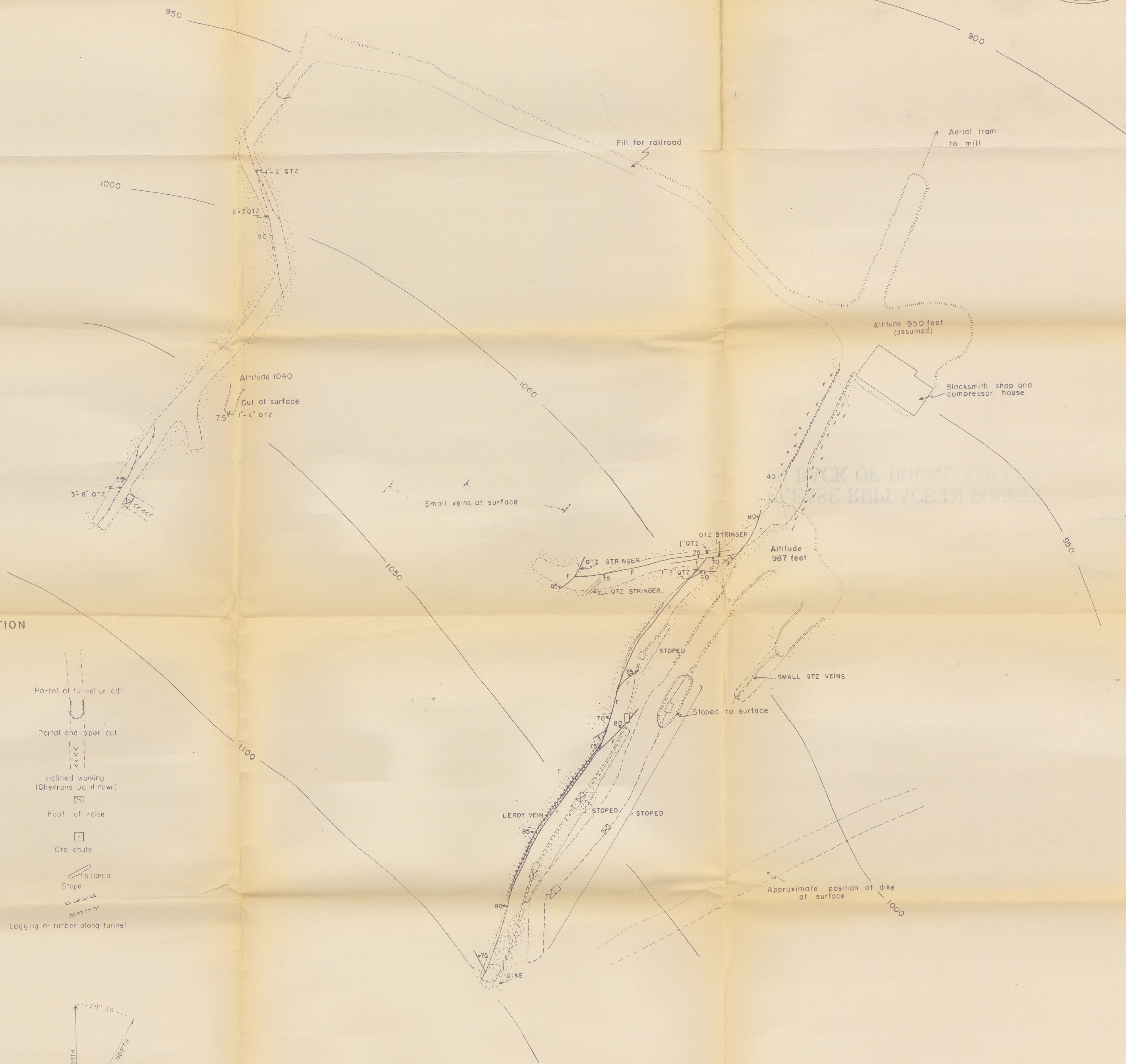
Map of workings and geology of the Leroy Mine
