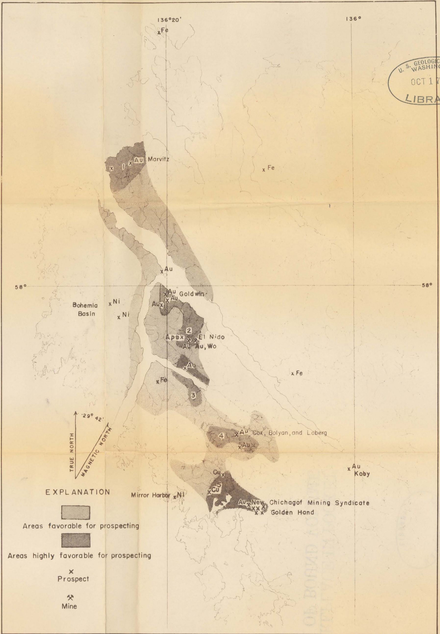
Figure 8. Map showing areas considered favorable for prospecting and location of mines and prospects.
