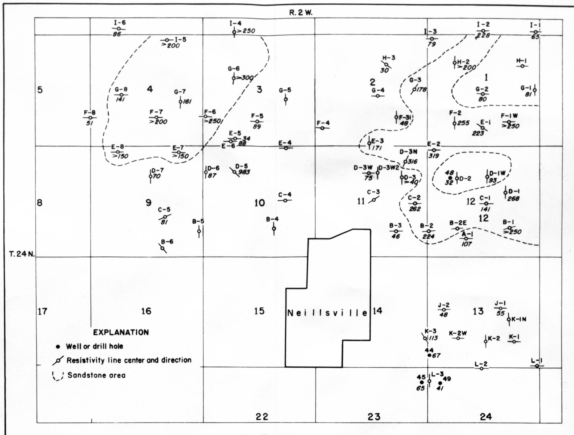
Figure 3.- Resistivity line centers, directions, and thicknesses of sandstone.
