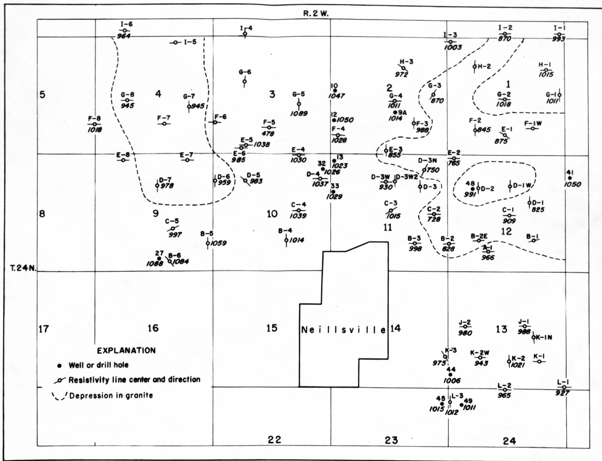
Figure 4.- Resistivity line centers, directions, and altitudes on granite.
