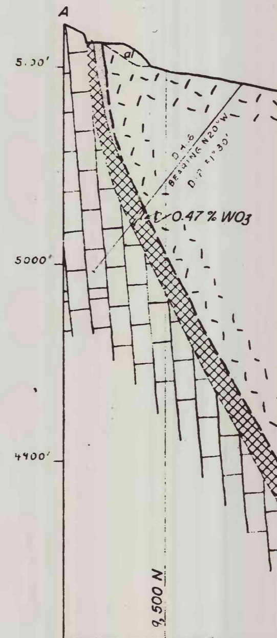
Geologic sections A-A', B-B', C-C' Nevada Scheelite mine
