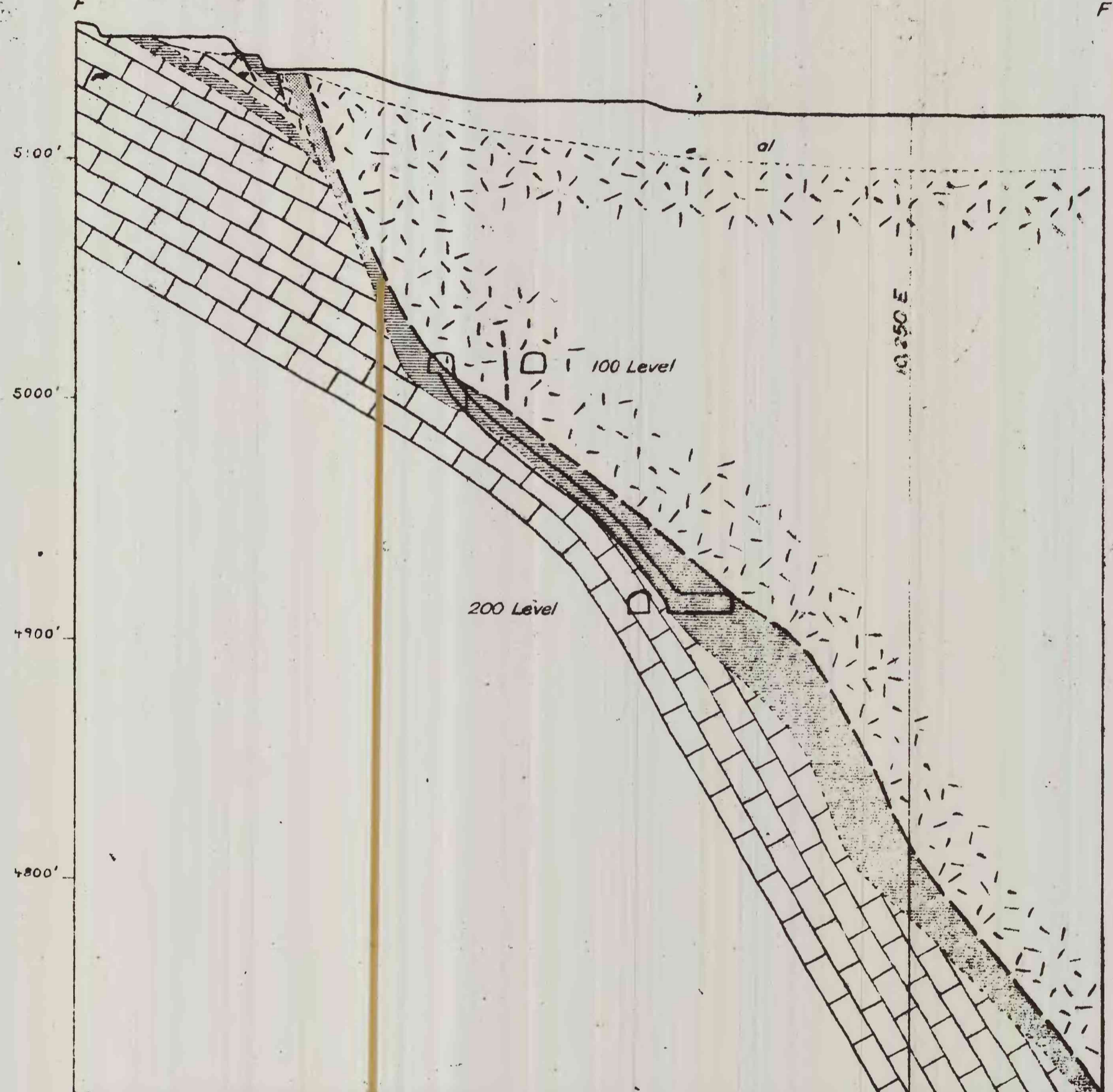
Geologic sections D-D', E-E', and F-F' Nevada Scheelite mine
